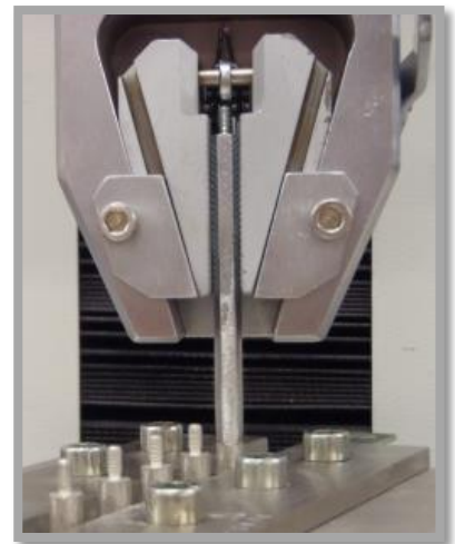
Checking fixture Pull Strength
