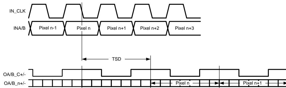
Figure 11. Single In Single Out / Dual In Dual Out Latency
