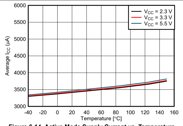
Figure 6-14. Active Mode Supply Current vs. Temperature
