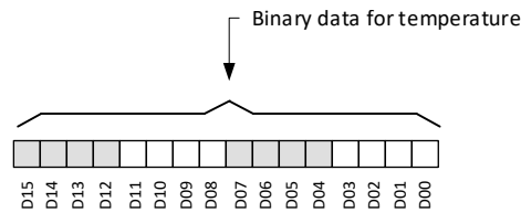
Figure 7-6. Temperature Sensor Data Definition
