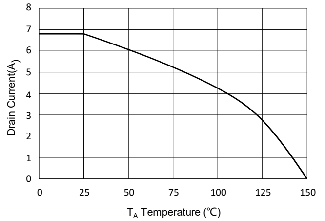
Fig.10 - Drain Current
