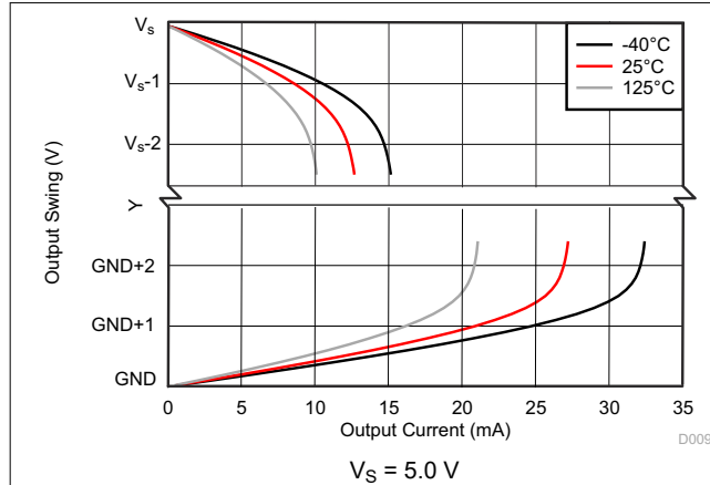
Figure 6-13. Output Voltage Swing vs. Output Current
