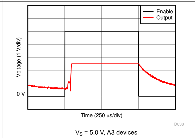
Figure 6-28. Enable and Disable Response
