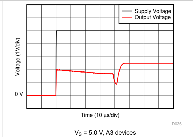
Figure 6-26. Start-Up Response
