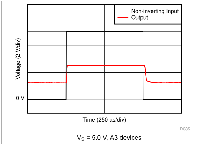
Figure 6-25. Noninverting Differential Input Overload
