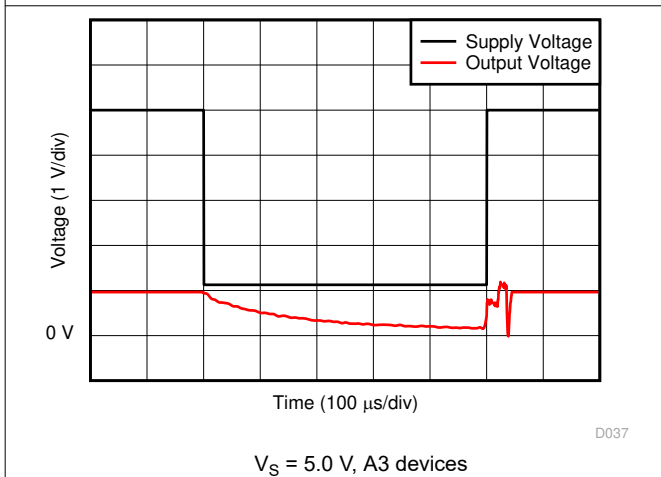
Figure 6-27. Brownout Recovery
