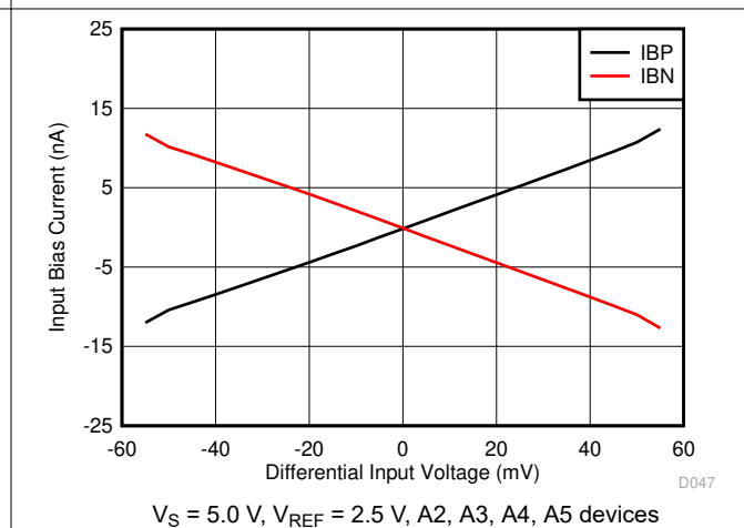
Figure 6-30. I_{B+} and I_{B-} vs. Differential Input Voltage
