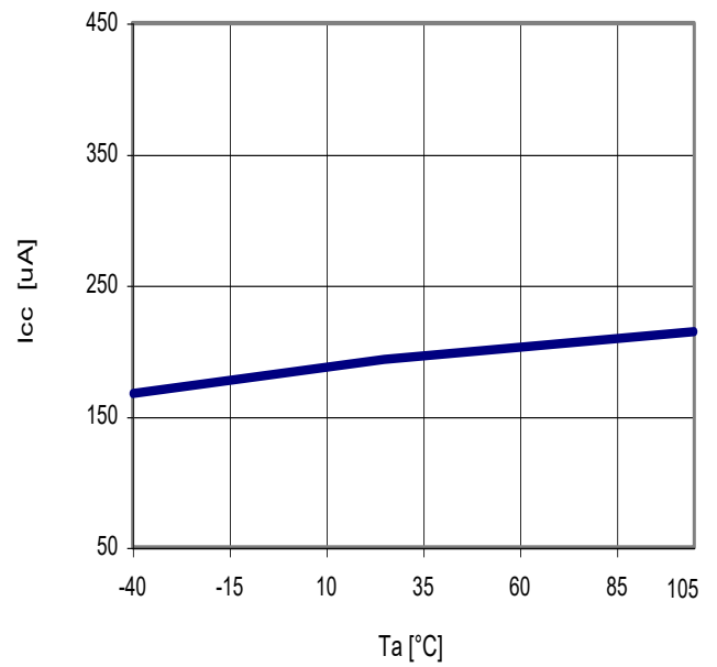
Fig.22 T_a - I_{CC}
