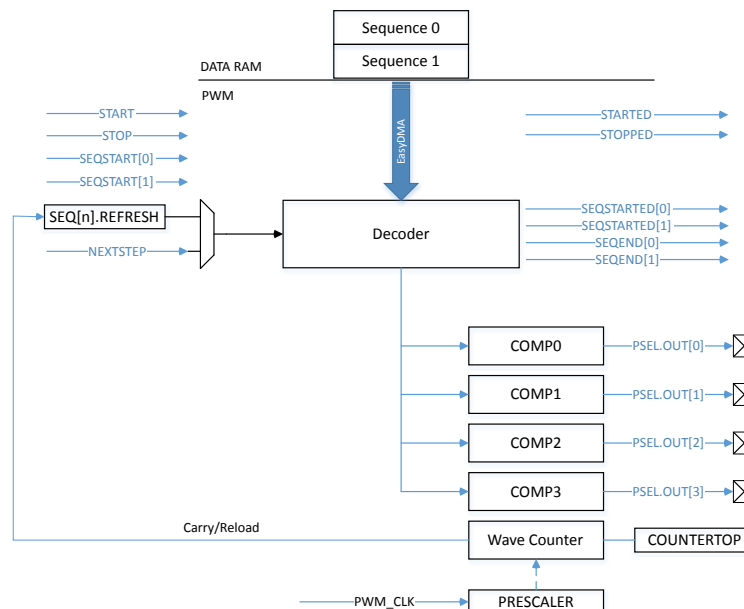
Figure 49: PWM module
