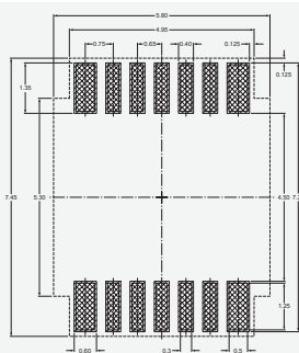
TSSOP14 (SOT402-1)
