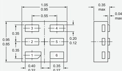
XSON6 (SOT1115)
