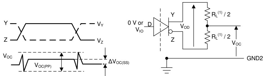
Figure 9-1. Driver Voltages
