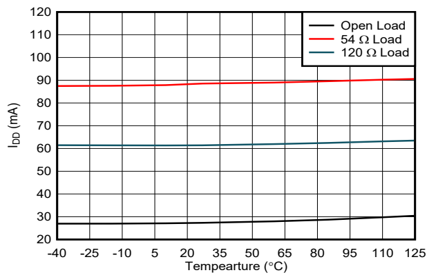
MODE = GND2 V_{DD} = 3.3\text{ V} \overline{RE} = \text{GND1} DE = V_{IO}
