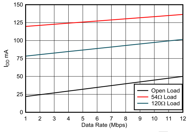
MODE = GND2 V_{DD} = 3.3\text{ V} \overline{RE} = \text{GND1} T_A = 25^\circ\text{C} DE = V_{IO}
