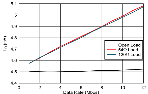
MODE = GND2 V_{DD} = 3.3\text{ V} \overline{RE} = \text{GND1} T_A = 25^\circ\text{C} DE = V_{IO}
