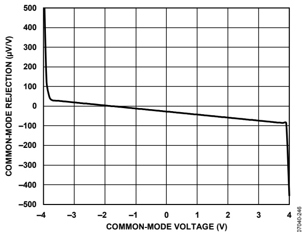
Figure 46. Common-Mode Rejection vs. Common-Mode Voltage
