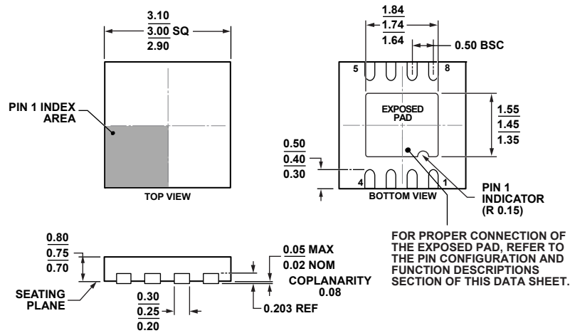
Figure 58. 8-Lead Lead Frame Chip Scale Package [LFCSP] 3 mm x 3 mm Body and 0.75 mm Package Height (CP-8-13) Dimensions shown in millimeters
