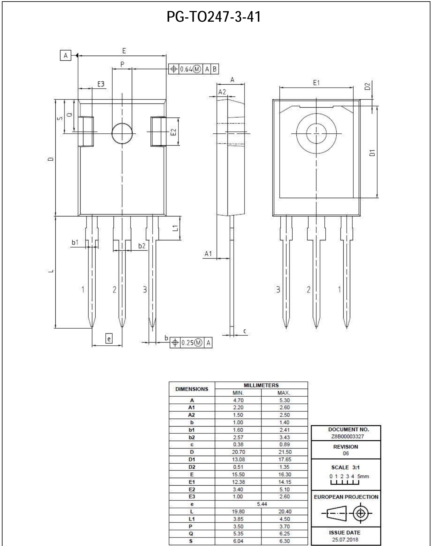
Figure 22 Package drawing
