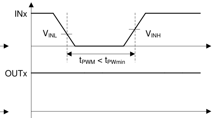
Figure 8-2. Deglitch Filter – Turn OFF
