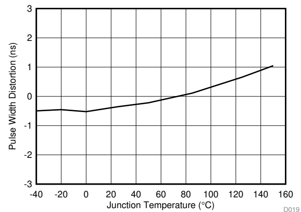
t_{PDHL} - t_{PDHL} Figure 7-21. Pulse Width Distortion
