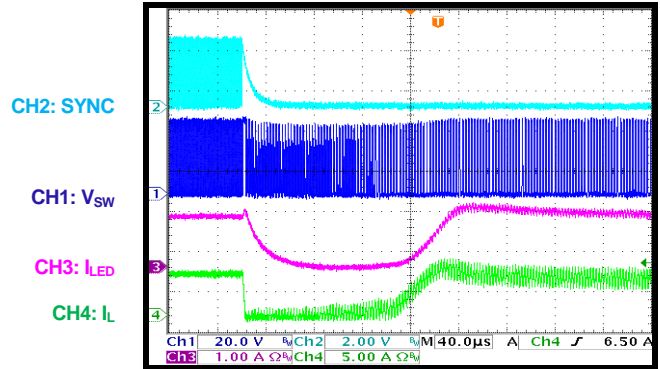
SYNC Out SYNC frequency = 2.2MHz
