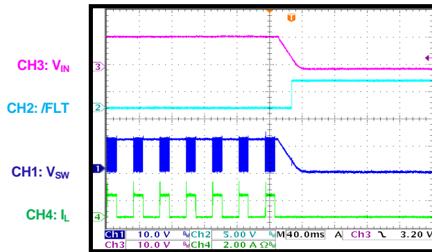
No Dimming LED+ to PGND short, shutdown
