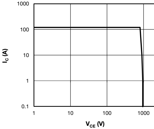
Fig. 17 - Trench IGBT Reverse BIAS SOA T_J = 150\text{ }^\circ\text{C} , I_C = 120\text{ A} , R_g = 10\ \Omega , V_{GE} = +15\text{V} / 0\text{V} , V_{CC} = 800\text{ V} , V_p = 1200\text{ V}
