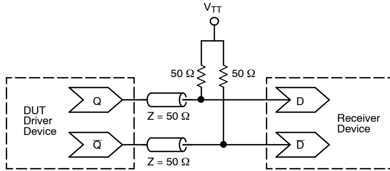
Figure 13. Typical Termination for Output Driver and Device Evaluation
