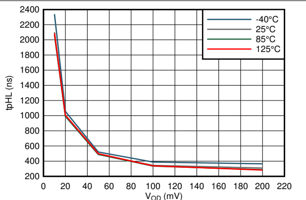
Figure 7-29. Propagation Delay High-Low vs Input Overdrive
