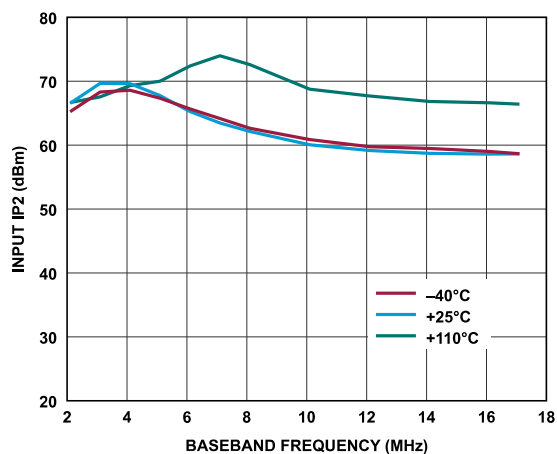
Figure 200. Receiver Input IP2 vs. Baseband Frequency, ADC = Low Power, f_1 = Baseband Frequency, f_2 = Baseband Frequency + 1 MHz, Gain Index = 255
