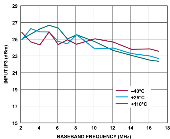
Figure 164. Receiver Input IP3 vs. Baseband Frequency, ADC = Low Power, f_1 = Baseband Frequency, f_2 = Baseband Frequency + 1 MHz, Gain Index = 255
