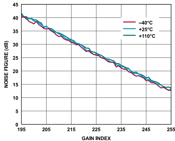
Figure 182. Receiver Noise Figure vs. Gain Index, Baseband Frequency = 5.6 MHz, ADC = High Performance
