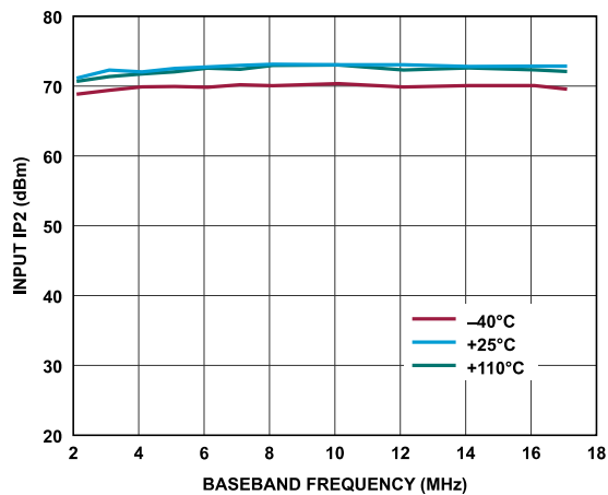
Figure 127. Receiver Input IP2 vs. Baseband Frequency, ADC = High Performance, f_1 = Baseband Frequency, f_2 = Baseband Frequency + 1 MHz, Gain Index = 255
