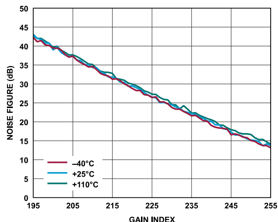
Figure 216. Receiver Noise Figure vs. Gain Index, Baseband Frequency = 2.1 kHz, ADC = High Performance
