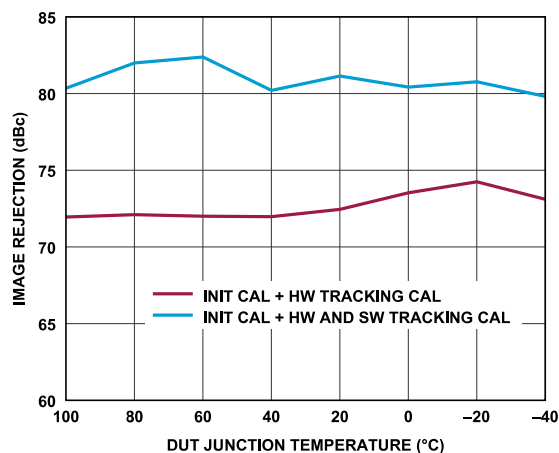
Figure 115. Receiver Image Rejection vs. DUT Junction Temperature (High to Low), Tone 1 Baseband Frequency = -5.1 MHz, Tone 2 Baseband Frequency = 13.9 MHz, ADC = Low Power, P_{OUT} = -11.1 dBFS
