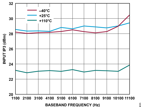
Figure 274. Receiver Input IP3 vs. Baseband Frequency, ADC = High Performance, f_1 = Baseband Frequency + 1 MHz, f_2 = Baseband Frequency + 2 MHz, Gain Index = 255, First-Order TIA with f_{3dB} = 4 MHz, P_{OUT} = -15.1 dBFS at -40°C and +25°C, P_{OUT} = -18.1 dBFS at +110°C
