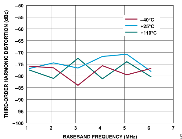
Figure 57. Receiver Third-Order Harmonic Distortion vs. Baseband Frequency, Gain Index = 255, ADC = Low Power
