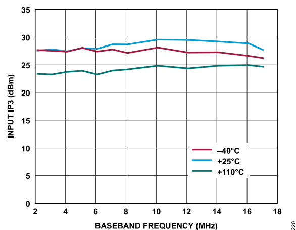
Figure 125. Receiver Input IP3 vs. Baseband Frequency, ADC = High Performance, f_1 = Baseband Frequency, f_2 = Baseband Frequency + 1 MHz, Gain Index = 255
