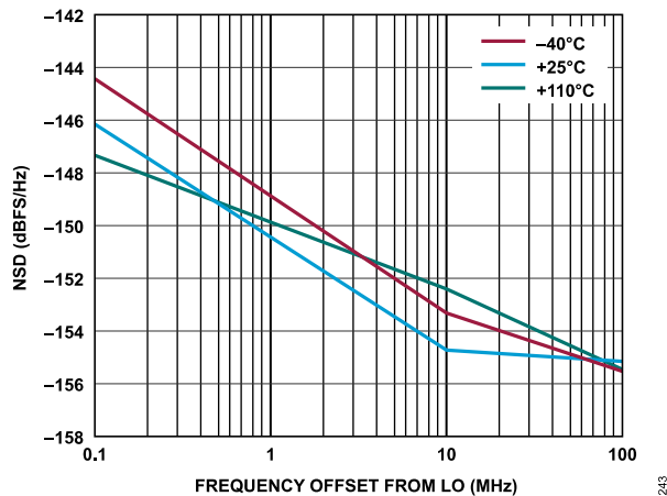
Figure 141. Transmitter NSD vs. Frequency Offset from LO, Baseband Frequency = 5.6 MHz, Transmitter Channel = Ch1
