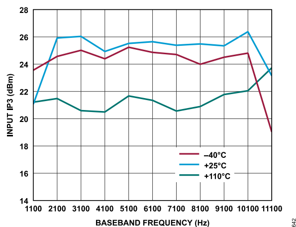
Figure 321. Receiver Input IP3 vs. Baseband Frequency, ADC = Low Power, f_1 = Baseband Frequency + 1 MHz, f_2 = Baseband Frequency + 2 MHz, Gain Index = 255, First-Order TIA with f_{1dB} = 4 MHz, P_{OUT} = -12.6 dBFS at -40°C and +25°C, P_{OUT} = -15.6 dBFS at +110°C
