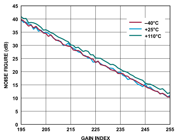
Figure 44. Receiver Noise Figure vs. Gain Index, Baseband Frequency = 5.6 MHz, ADC = High Performance
