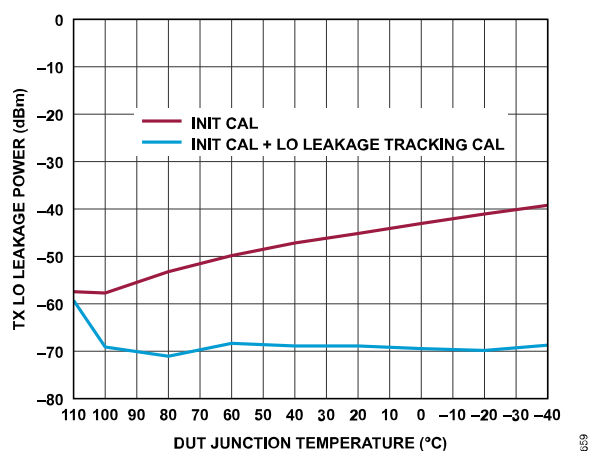
Figure 177. Transmitter LO Leakage Power vs. DUT Junction Temperature (High to Low), Baseband Frequency = 4 MHz, Backoff = 0.5 dBFS, Attenuation Code = 0
