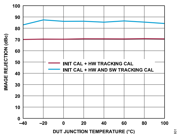
Figure 13. Receiver Image Rejection vs. DUT Junction Temperature (Low to High), Tone 1 Baseband Frequency = -5.1 MHz, Tone 2 Baseband Frequency = 13.9 MHz, ADC = Low Power, P_{OUT} = -15.1 dBFS
