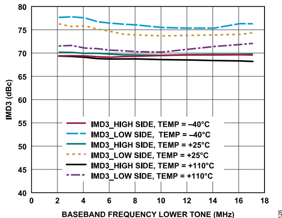
Figure 41. Transmitter Third-Order Intermodulation Distortion (IMD3) vs. Baseband Frequency, Transmitter Attenuation Code = 0, f_1 = Baseband Frequency, f_2 = Baseband Frequency + 1 MHz
