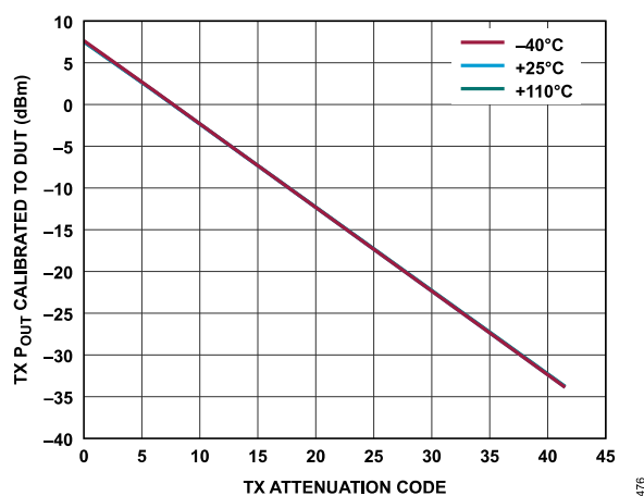
Figure 324. Transmitter Absolute Power vs. Transmitter Attenuation Code, Baseband Frequency = 2.1 kHz, Backoff = 0.2 dBFS
