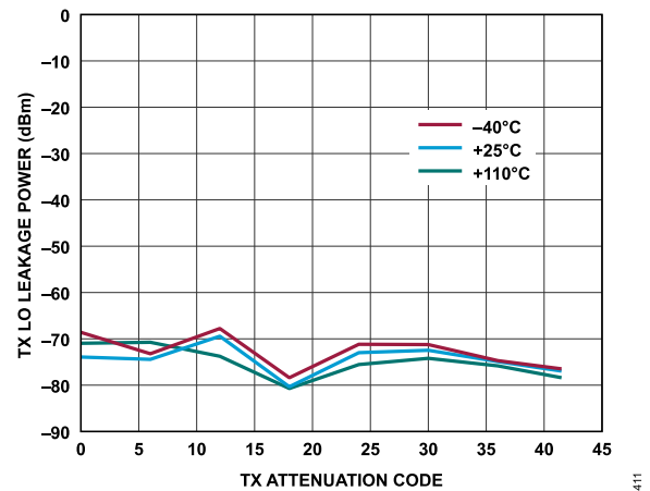
Figure 282. Transmitter LO Leakage Power vs. Transmitter Attenuation Code, Baseband Frequency = 2.1 kHz, Backoff = 6 dBFS, Initialization Calibration Only
