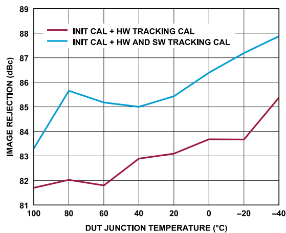
Figure 82. Receiver Image Rejection vs. DUT Junction Temperature (High to Low), Tone 1 Baseband Frequency = -5.1 MHz, Tone 2 Baseband Frequency = 13.9 MHz, ADC = Low Power, P_{OUT} = -11.1 dBFS
