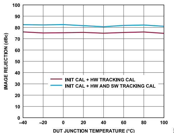
Figure 113. Receiver Image Rejection vs. DUT Junction Temperature (Low to High), Tone 1 Baseband Frequency = -5.1 MHz, Tone 2 Baseband Frequency = 13.9 MHz, ADC = Low Power, P_{OUT} = -11.1 dBFS
