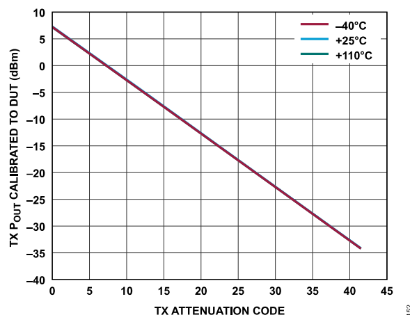
Figure 63. Transmitter Absolute Power vs. Transmitter Attenuation Code, Baseband Frequency = 18 MHz, Backoff = 0.2 dBFS
