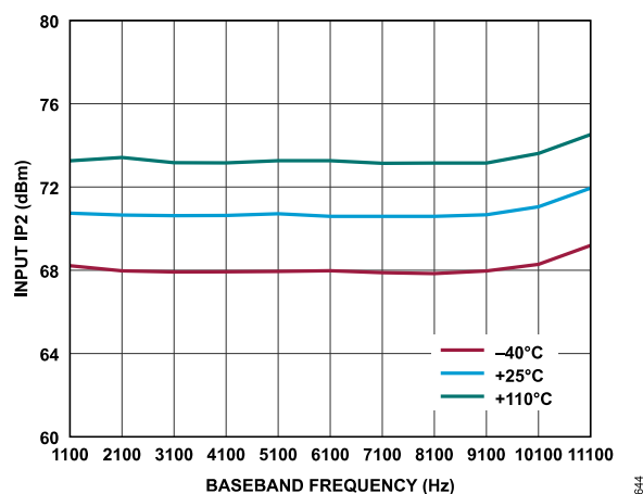
Figure 323. Receiver Input IP2 vs. Baseband Frequency, ADC = Low Power, f_1 = Baseband Frequency + 1 MHz, f_2 = Baseband Frequency + 2 MHz, Gain Index = 255, First-Order TIA with f_{3dB} = 4 MHz, P_{OUT} = -6.6 dBFS
