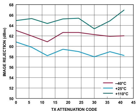
Figure 100. Transmitter Image Rejection vs. Transmitter Attenuation Code, Baseband Frequency = 18 MHz, Backoff = 0.2 dBFS, Initialization Calibration Only
