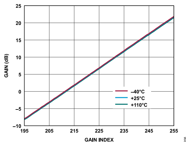
Figure 109. Receiver Absolute Gain (Complex) vs. Gain Index, Baseband Frequency = 5.6 MHz, ADC = High Performance, P_{OUT} = -9.6 dBFS
