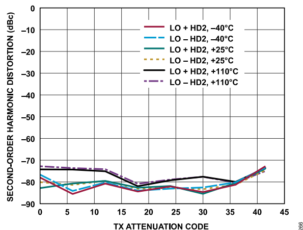
Figure 174. Transmitter Second-Order Harmonic Distortion vs. Transmitter Attenuation Code, Baseband Frequency = 18 MHz, Backoff = 0.2 dBFS
