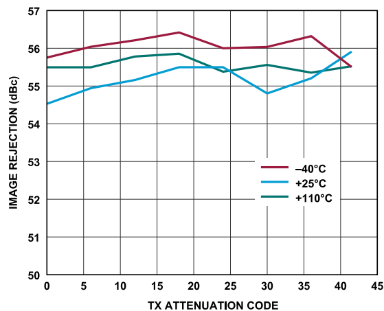
Figure 34. Transmitter Image Rejection vs. Transmitter Attenuation Code, Baseband Frequency = 18 MHz, Backoff = 0.2 dBFS, Initialization Calibration Only
