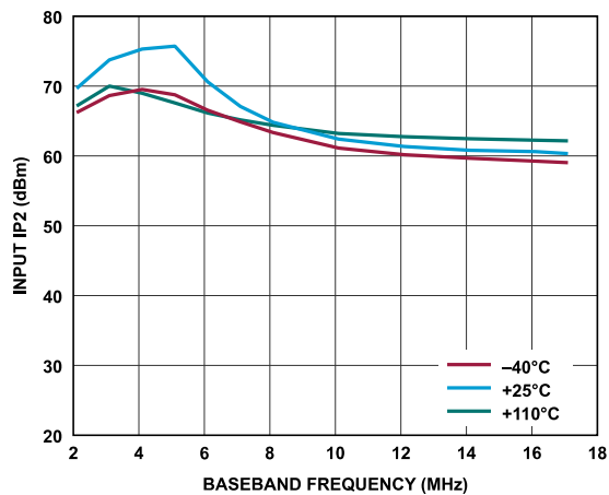
Figure 199. Receiver Input IP2 vs. Baseband Frequency, ADC = High Performance, f_1 = Baseband Frequency, f_2 = Baseband Frequency + 1 MHz, Gain Index = 255
