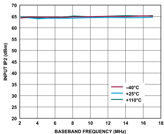
Figure 128. Receiver Input IP2 vs. Baseband Frequency, ADC = Low Power, f_1 = Baseband Frequency, f_2 = Baseband Frequency + 1 MHz, Gain Index = 255
