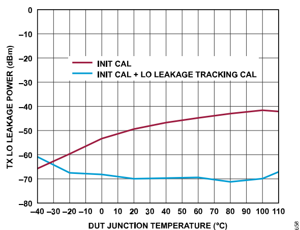
Figure 176. Transmitter LO Leakage Power vs. DUT Junction Temperature (Low to High), Baseband Frequency = 4 MHz, Backoff = 0.5 dBFS, Attenuation Code = 0
