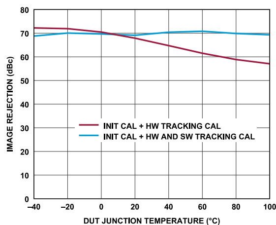
Figure 150. Receiver Image Rejection vs. DUT Junction Temperature (Low to High), Tone 1 Baseband Frequency = -5.1 MHz, Tone 2 Baseband Frequency = 13.9 MHz, ADC = High Performance, P_{OUT} = -11.1 dBFS
