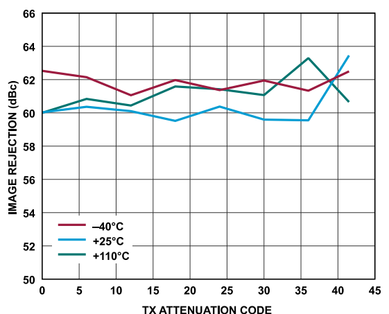
Figure 133. Transmitter Image Rejection vs. Transmitter Attenuation Code, Baseband Frequency = 18 MHz, Backoff = 0.2 dBFS, Initialization Calibration Only
