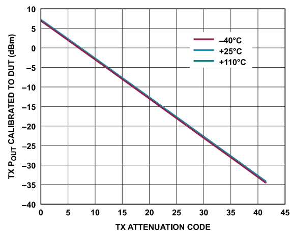
Figure 231. Transmitter Absolute Power vs. Transmitter Attenuation Code, Baseband Frequency = 2.1 kHz, Backoff = 0.2 dBFS
