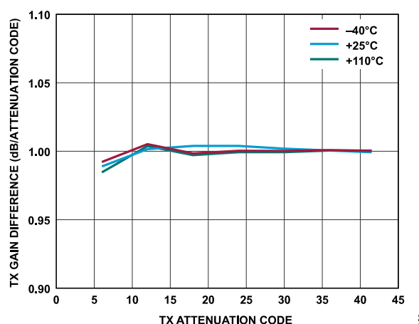
Figure 97. Transmitter Attenuation Delta (Error) vs. Transmitter Attenuation Code, Baseband Frequency = 18 MHz, Backoff = 0.2 dBFS
