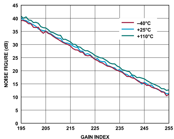
Figure 110. Receiver Noise Figure vs. Gain Index, Baseband Frequency = 5.6 MHz, ADC = High Performance
