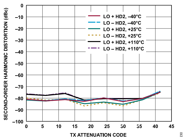
Figure 135. Transmitter Second-Order Harmonic Distortion vs. Transmitter Attenuation Code, Baseband Frequency = 18 MHz, Backoff = 0.2 dBFS
