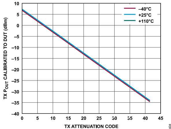
Figure 273. Transmitter Absolute Power vs. Transmitter Attenuation Code, Baseband Frequency = 2.1 kHz, Backoff = 0.2 dBFS
