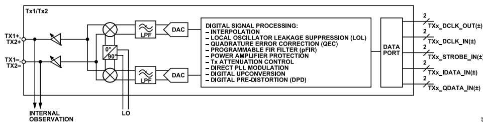
Figure 360. Transmitter Architecture
