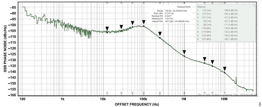
Figure 358. Internal Local Oscillator Phase Noise at 3500 MHz LO
