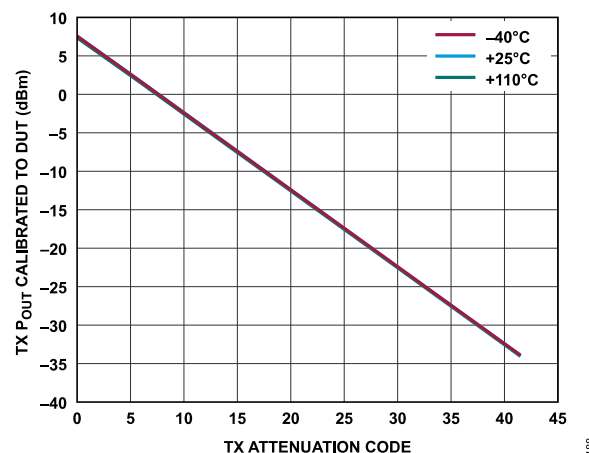
Figure 96. Transmitter Absolute Power vs. Transmitter Attenuation Code, Baseband Frequency = 18 MHz, Backoff = 0.2 dBFS
