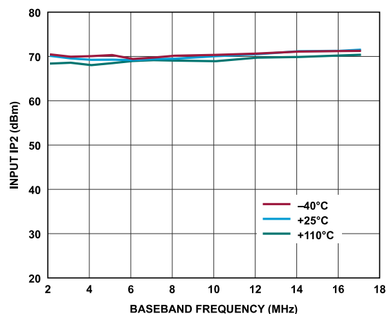
Figure 95. Receiver Input IP2 vs. Baseband Frequency, ADC = Low Power, f_1 = Baseband Frequency, f_2 = Baseband Frequency + 1 MHz, Gain Index = 255
