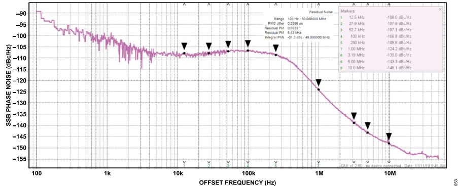
Figure 357. Internal Local Oscillator Phase Noise at 2400 MHz LO
