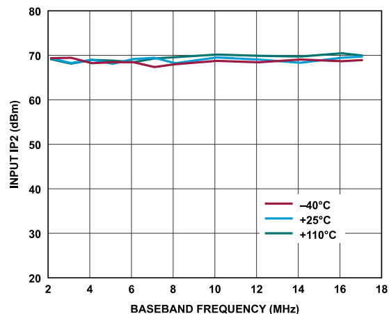
Figure 28. Receiver Input IP2 vs. Baseband Frequency, ADC = Low Power, f_1 = Baseband Frequency, f_2 = Baseband Frequency + 1 MHz, Gain Index = 255
