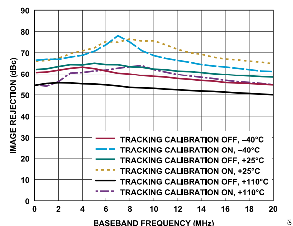
Figure 65. Transmitter Image Rejection vs. Baseband Frequency, Tracking Calibration On vs. Tracking Calibration Off, Transmitter Attenuation Code = 0
