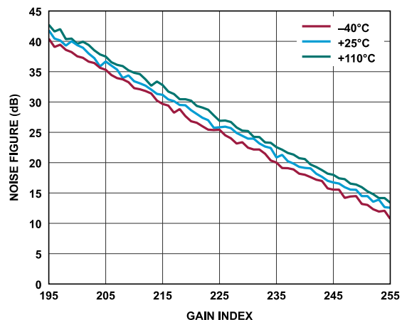
Figure 111. Receiver Noise Figure vs. Gain Index, Baseband Frequency = 5.6 MHz, ADC = Low Power
