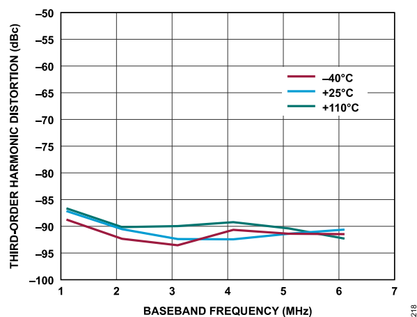
Figure 121. Receiver Third-Order Harmonic Distortion vs. Baseband Frequency, Gain Index = 255, ADC = High Performance
