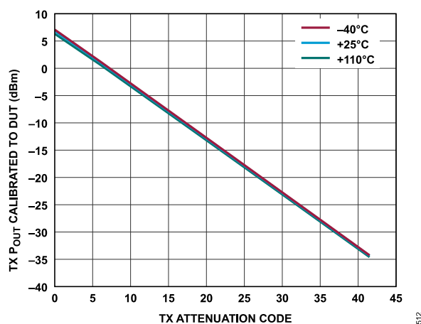
Figure 347. Transmitter Absolute Power vs. Transmitter Attenuation Code, Baseband Frequency = 2.1 kHz, Backoff = 0.2 dBFS
