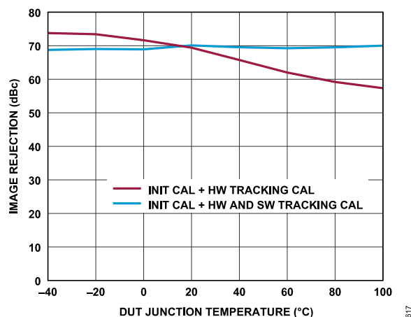
Figure 151. Receiver Image Rejection vs. DUT Junction Temperature (Low to High), Tone 1 Baseband Frequency = -5.1 MHz, Tone 2 Baseband Frequency = 13.9 MHz, ADC = Low Power, P_{OUT} = -11.1 dBFS
