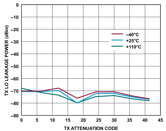
Figure 305. Transmitter LO Leakage Power vs. Transmitter Attenuation Code, Baseband Frequency = 2.1 kHz, Backoff = 6 dBFS, Initialization Calibration Only
