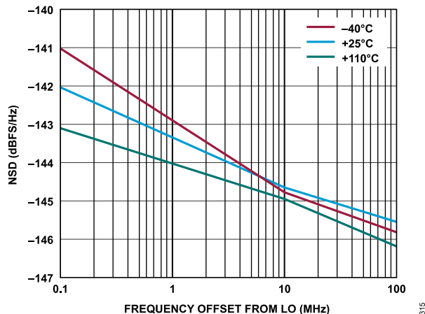
Figure 213. Transmitter NSD vs. Frequency Offset from LO, Baseband Frequency = 5.6 MHz, Transmitter Channel = Ch1
