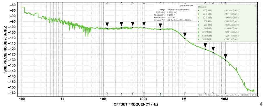
Figure 359. Internal Local Oscillator Phase Noise at 5800 MHz LO
