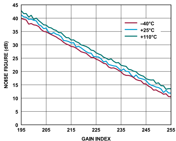
Figure 45. Receiver Noise Figure vs. Gain Index, Baseband Frequency = 5.6 MHz, ADC = Low Power
