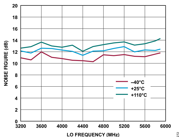
Figure 145. Receiver Noise Figure vs. LO Frequency, Baseband Frequency = 5.6 MHz, ADC = High Performance
