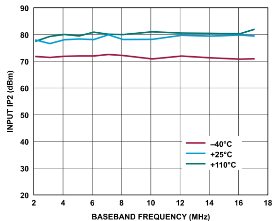
Figure 27. Receiver Input IP2 vs. Baseband Frequency, ADC = High Performance, f_1 = Baseband Frequency, f_2 = Baseband Frequency + 1 MHz, Gain Index = 255
