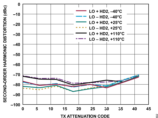
Figure 207. Transmitter Second-Order Harmonic Distortion vs. Transmitter Attenuation Code, Baseband Frequency = 18 MHz, Backoff = 0.2 dBFS
