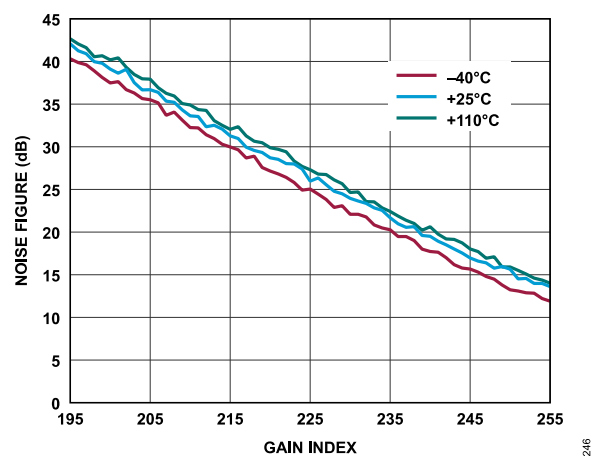
Figure 146. Receiver Noise Figure vs. Gain Index, Baseband Frequency = 5.6 MHz, ADC = Low Power
