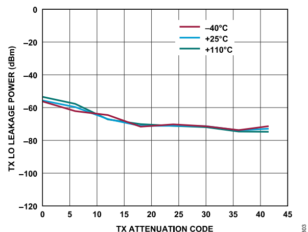
Figure 208. Transmitter LO Leakage Power vs. Transmitter Attenuation Code, Baseband Frequency = 18 MHz, Backoff = 6 dBFS, Initialization Calibration Only
