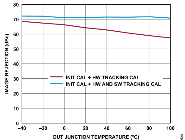
Figure 184. Receiver Image Rejection vs. DUT Junction Temperature (Low to High), Tone 1 Baseband Frequency = -5.1 MHz, Tone 2 Baseband Frequency = 13.9 MHz, ADC = High Performance, P_{OUT} = -11.1 dBFS
