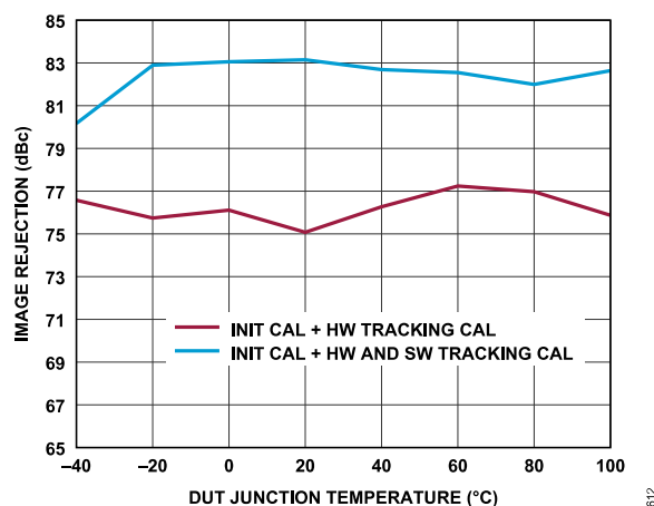
Figure 112. Receiver Image Rejection vs. DUT Junction Temperature (Low to High), Tone 1 Baseband Frequency = -5.1 MHz, Tone 2 Baseband Frequency = 13.9 MHz, ADC = High Performance, P_{OUT} = -11.1 dBFS
