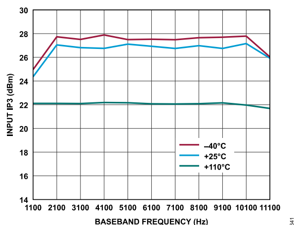
Figure 320. Receiver Input IP3 vs. Baseband Frequency, ADC = High Performance, f_1 = Baseband Frequency + 1 MHz, f_2 = Baseband Frequency + 2 MHz, Gain Index = 255, First-Order TIA with f_{1dB} = 4 MHz, P_{OUT} = -12.6 dBFS at -40°C and +25°C, P_{OUT} = -15.6 dBFS at +110°C
