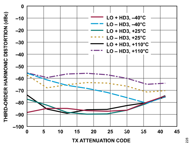
Figure 134. Transmitter Third-Order Harmonic Distortion vs. Transmitter Attenuation Code, Baseband Frequency = 18 MHz, Backoff = 0.2 dBFS
