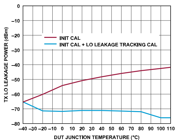
Figure 104. Transmitter LO Leakage Power vs. DUT Junction Temperature (Low to High), Baseband Frequency = 4 MHz, Backoff = 0.5 dBFS, Attenuation Code = 0
