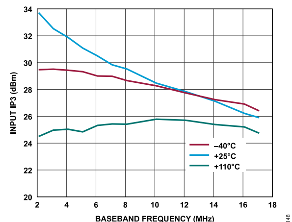
Figure 59. Receiver Input IP3 vs. Baseband Frequency, ADC = High Performance, f_1 = Baseband Frequency, f_2 = Baseband Frequency + 1 MHz, Gain Index = 255
