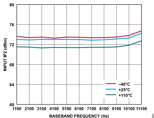
Figure 322. Receiver Input IP2 vs. Baseband Frequency, ADC = High Performance, f_1 = Baseband Frequency + 1 MHz, f_2 = Baseband Frequency + 2 MHz, Gain Index = 255, First-Order TIA with f_{3dB} = 4 MHz, P_{OUT} = -6.6 dBFS
