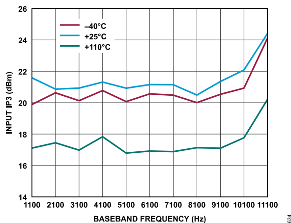
Figure 275. Receiver Input IP3 vs. Baseband Frequency, ADC = Low Power, f_1 = Baseband Frequency + 1 MHz, f_2 = Baseband Frequency + 2 MHz, Gain Index = 255, First-Order TIA with f_{3dB} = 4 MHz, P_{OUT} = -15.1 dBFS at -40°C and +25°C, P_{OUT} = -18.1 dBFS at +110°C
