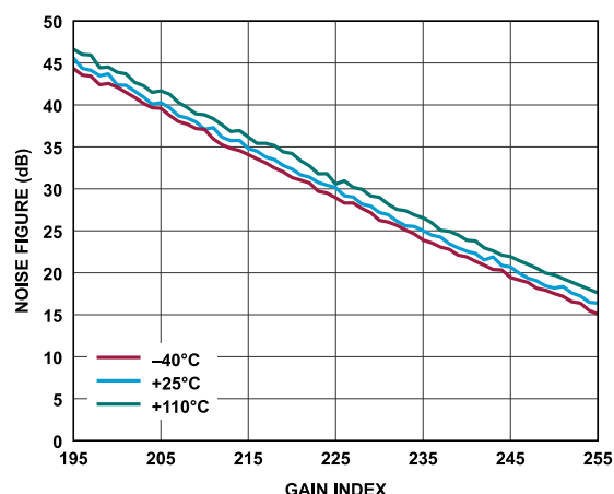
Figure 217. Receiver Noise Figure vs. Gain Index, Baseband Frequency = 2.1 kHz, ADC = Low Power
