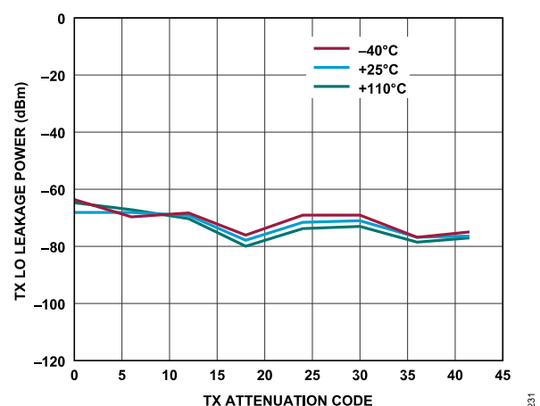
Figure 136. Transmitter LO Leakage Power vs. Transmitter Attenuation Code, Baseband Frequency = 18 MHz, Backoff = 6 dBFS, Initialization Calibration Only
