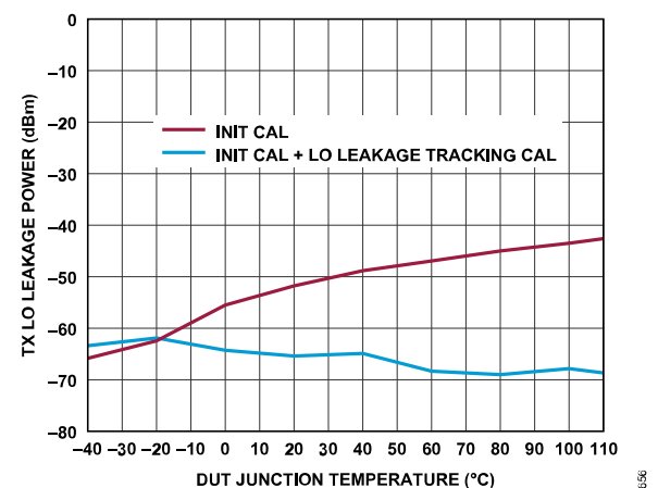
Figure 137. Transmitter LO Leakage Power vs. DUT Junction Temperature (Low to High), Baseband Frequency = 4 MHz, Backoff = 0.5 dBFS, Attenuation Code = 0
