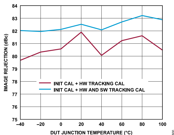
Figure 12. Receiver Image Rejection vs. DUT Junction Temperature (Low to High), Tone 1 Baseband Frequency = -5.1 MHz, Tone 2 Baseband Frequency = 13.9 MHz, ADC = High Performance, P_{OUT} = -15.1 dBFS
