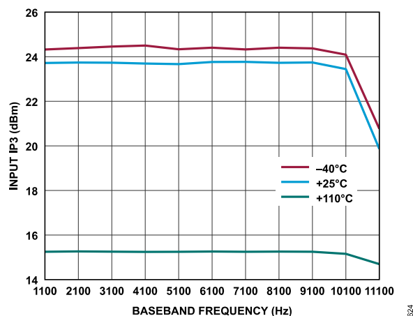
Figure 227. Receiver Input IP3 vs. Baseband Frequency, ADC = High Performance, f_1 = Baseband Frequency + 1 MHz, f_2 = Baseband Frequency + 2 MHz, Gain Index = 255, First-Order TIA with f_{1dB} = 4 MHz, P_{OUT} = -15.1 dBFS at -40°C and +25°C, P_{OUT} = -18.1 dBFS at +110°C
