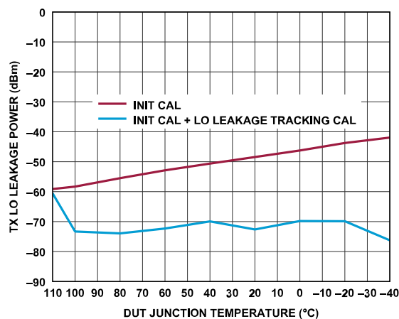
Figure 39. Transmitter LO Leakage Power vs. DUT Junction Temperature (High to Low), Baseband Frequency = 4 MHz, Backoff = 0.5 dBFS, Attenuation Code = 0
