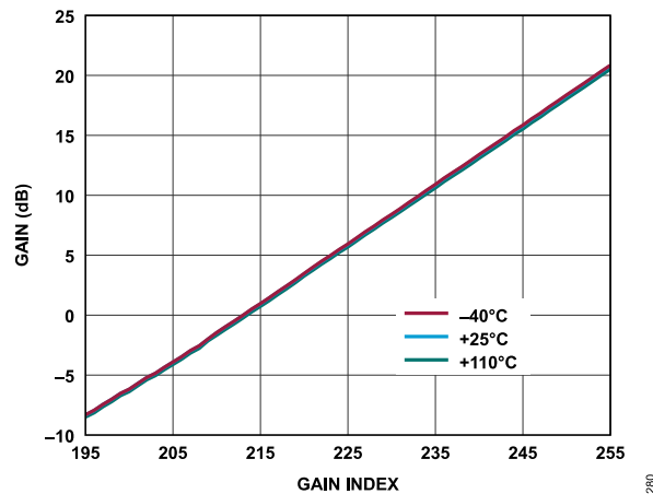
Figure 181. Receiver Absolute Gain (Complex) vs. Gain Index, Baseband Frequency = 5.6 MHz, ADC = High Performance, P_{OUT} = -9.6 dBFS
