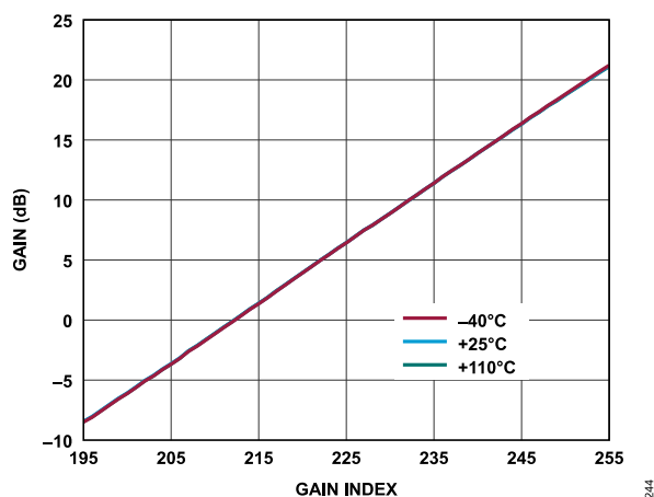
Figure 142. Receiver Absolute Gain (Complex) vs. Gain Index, Baseband Frequency = 5.6 MHz, ADC = High Performance, P_{OUT} = -9.6 dBFS
