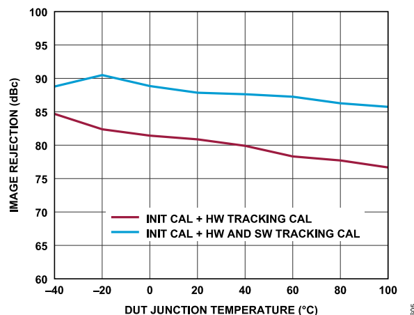
Figure 47. Receiver Image Rejection vs. DUT Junction Temperature (Low to High), Tone 1 Baseband Frequency = -5.1 MHz, Tone 2 Baseband Frequency = 13.9 MHz, ADC = Low Power, P_{OUT} = -11.1 dBFS
