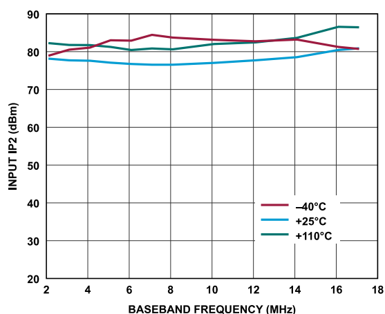
Figure 61. Receiver Input IP2 vs. Baseband Frequency, ADC = High Performance, f_1 = Baseband Frequency, f_2 = Baseband Frequency + 1 MHz, Gain Index = 255
