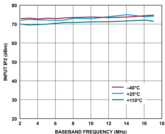
Figure 62. Receiver Input IP2 vs. Baseband Frequency, ADC = Low Power, f_1 = Baseband Frequency, f_2 = Baseband Frequency + 1 MHz, Gain Index = 255
