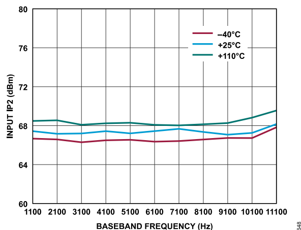
Figure 345. Receiver Input IP2 vs. Baseband Frequency, ADC = High Performance, f_1 = Baseband Frequency + 1 MHz, f_2 = Baseband Frequency + 2 MHz, Gain Index = 255, First-Order TIA with f_{3dB} = 4 MHz, P_{OUT} = -6.6 dBFS
