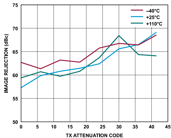
Figure 302. Transmitter Image Rejection vs. Transmitter Attenuation Code, Baseband Frequency = 2.1 kHz, Backoff = 0.2 dBFS, Initialization Calibration Only
