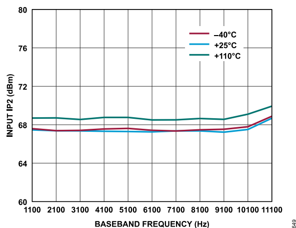
Figure 346. Receiver Input IP2 vs. Baseband Frequency, ADC = Low Power, f_1 = Baseband Frequency + 1 MHz, f_2 = Baseband Frequency + 2 MHz, Gain Index = 255, First-Order TIA with f_{3dB} = 4 MHz, P_{OUT} = -6.6 dBFS
