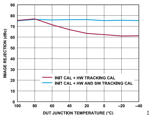
Figure 152. Receiver Image Rejection vs. DUT Junction Temperature (High to Low), Tone 1 Baseband Frequency = -5.1 MHz, Tone 2 Baseband Frequency = 13.9 MHz, ADC = High Performance, P_{OUT} = -11.1 dBFS
