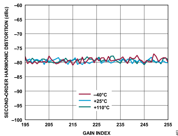
Figure 311. Receiver Second-Order Harmonic Distortion vs. Gain Index, Baseband Frequency = 2.1 kHz, ADC = High Performance
