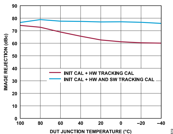
Figure 153. Receiver Image Rejection vs. DUT Junction Temperature (High to Low), Tone 1 Baseband Frequency = -5.1 MHz, Tone 2 Baseband Frequency = 13.9 MHz, ADC = Low Power, P_{OUT} = -11.1 dBFS
