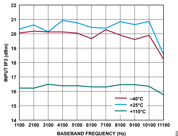
Figure 228. Receiver Input IP3 vs. Baseband Frequency, ADC = Low Power, f_1 = Baseband Frequency + 1 MHz, f_2 = Baseband Frequency + 2 MHz, Gain Index = 255, First-Order TIA with f_{1dB} = 4 MHz, P_{OUT} = -15.1 dBFS at -40°C and +25°C, P_{OUT} = -18.1 dBFS at +110°C
