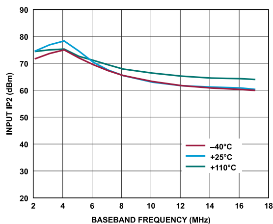
Figure 165. Receiver Input IP2 vs. Baseband Frequency, ADC = High Performance, f_1 = Baseband Frequency, f_2 = Baseband Frequency + 1 MHz, Gain Index = 255
