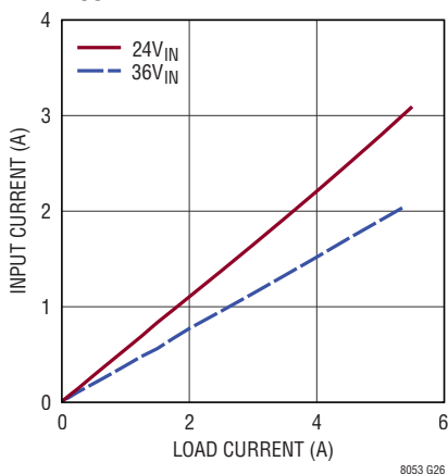
LTM8053 Input vs Load Current V_{OUT} = 12\text{V} , \text{BIAS} = 5\text{V}
