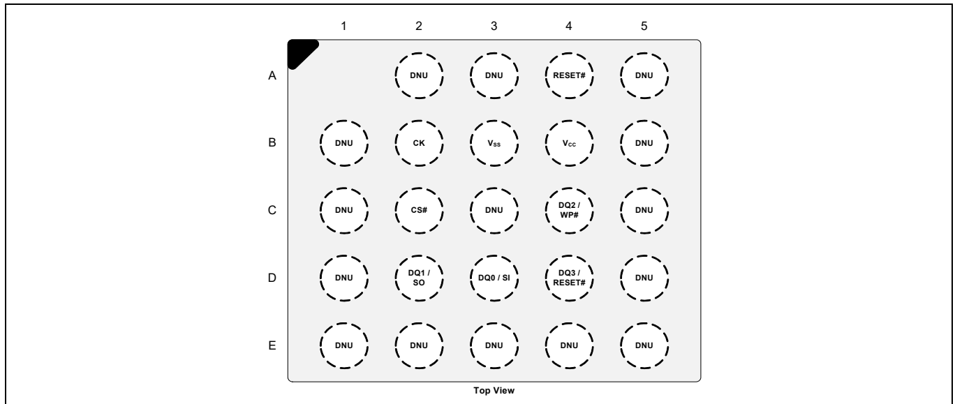
Figure 1 24-ball BGA pinout configuration
