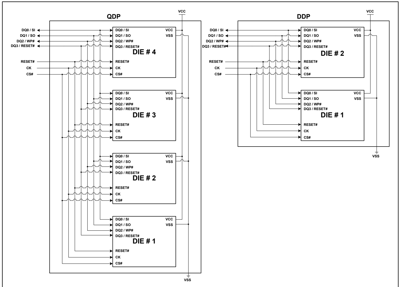
Figure 3 MCP diagram
