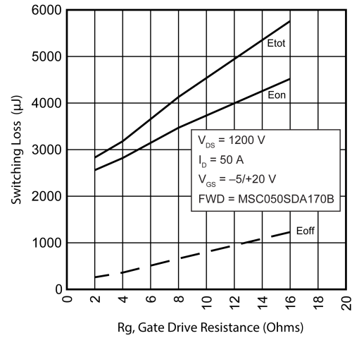
Figure 18 • Switching Energy vs. R_g
