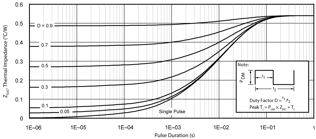
Figure 21 • Maximum Transient Thermal Impedance
