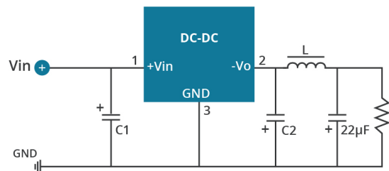
Figure 5 Negative Output Ripple Reduction Circuit
