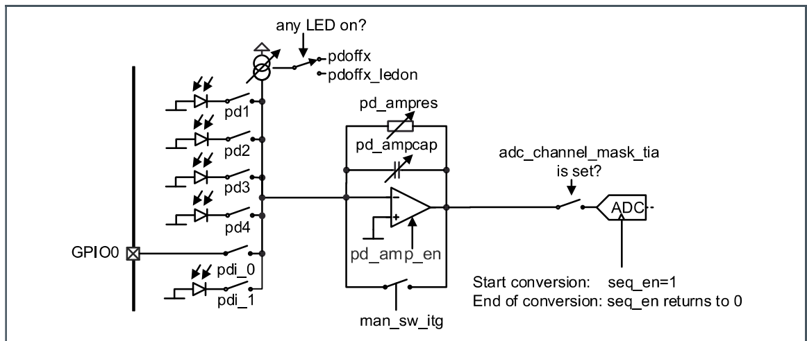
Figure 39: Optical Frontend
