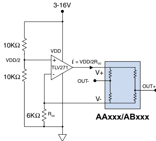
Figure 11. Constant-current supply.
