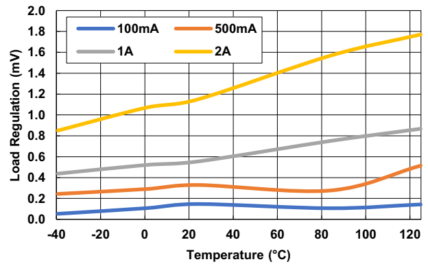
Figure 102. Load Regulation vs Temperature ( V_{IN} = 2.7V , V_{OUT} = 0.8V , \Delta I_{OUT} = 1mA to 2A )
