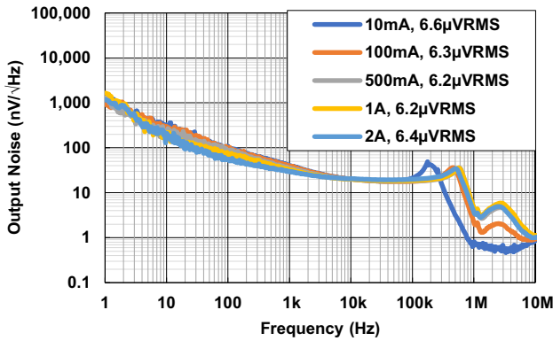
Figure 11. Output Noise vs Frequency for Various I_{OUT} ( V_{IN} = V_{OUT} + 1\text{V} , I_{OUT} = 2\text{A} )
