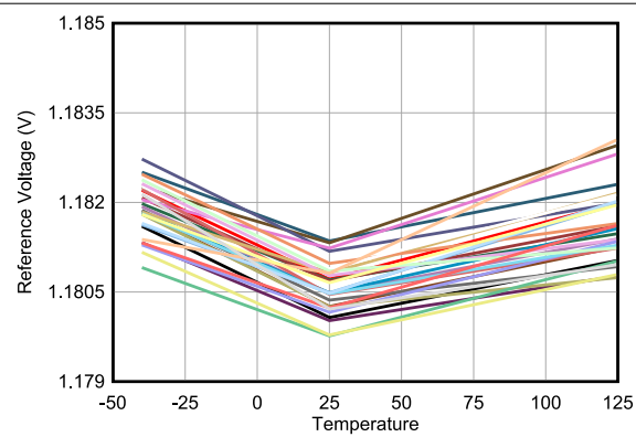
Figure 6-29. Internal Reference Voltage Temperature Drift
