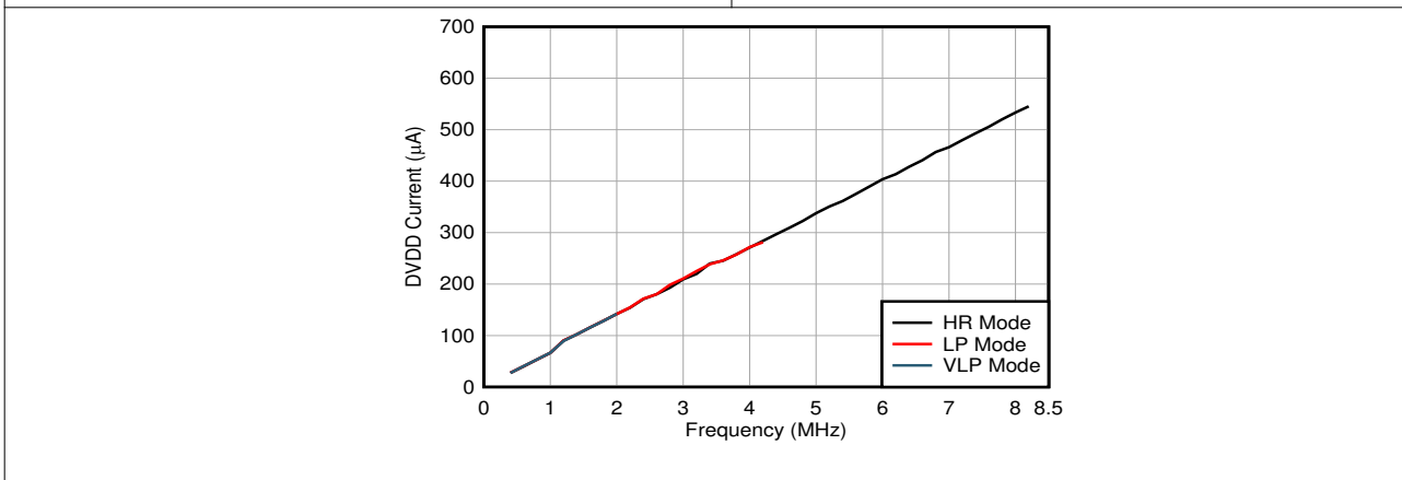
Figure 6-31. AVDD Current vs CLKIN Frequency
