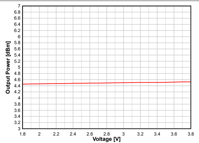
Figure 8-22. Output Power vs. Supply Voltage (VDD5) (BLE 1 Mbps, 2.44 GHz, +5 dBm)
