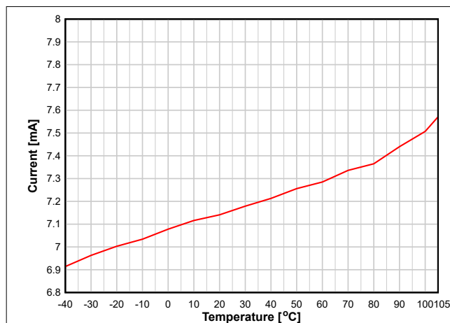
Figure 8-6. RX Current vs. Temperature (BLE 1 Mbps, 2.44 GHz)
