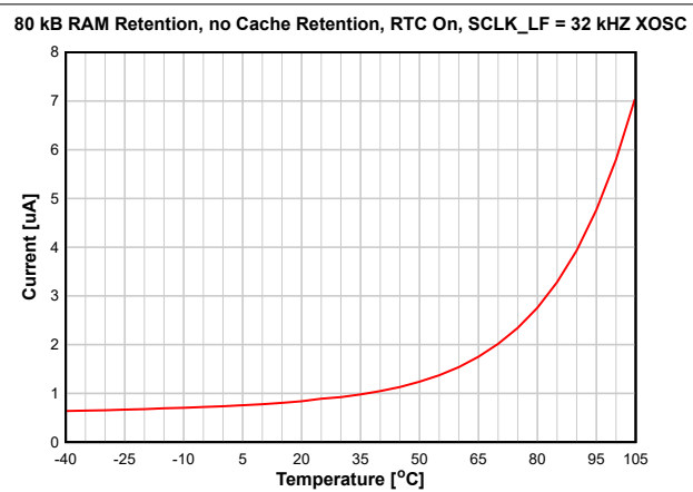
Figure 8-5. Standby Mode (MCU) Current vs. Temperature
