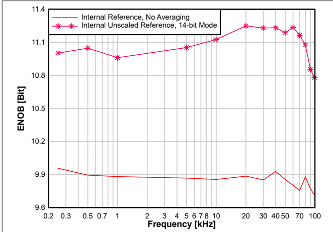
Figure 8-25. ENOB vs. Input Frequency
