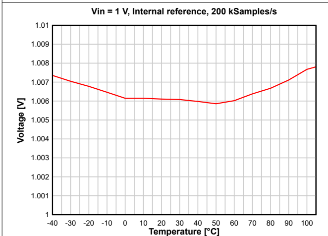
Figure 8-29. ADC Accuracy vs. Temperature
