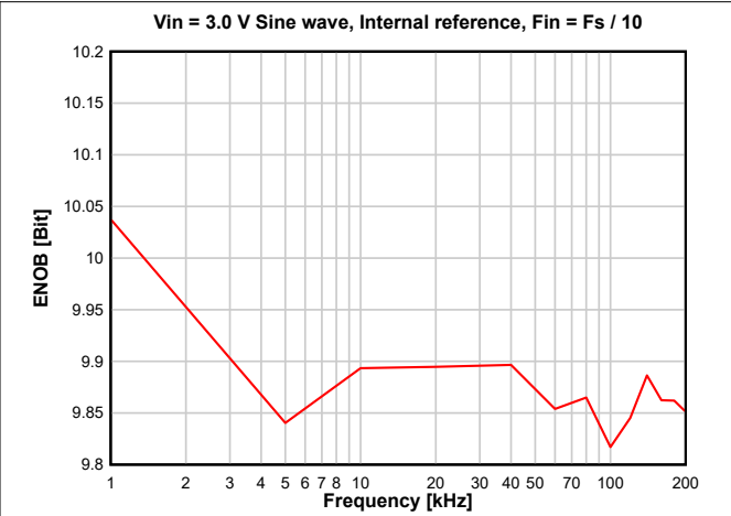
Figure 8-26. ENOB vs. Sampling Frequency
