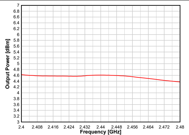
Figure 8-24. Output Power vs. Frequency (BLE 1 Mbps, +5 dBm)
