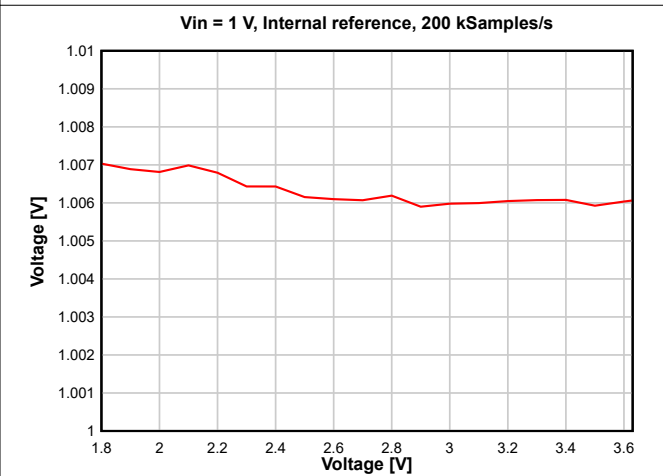
Figure 8-30. ADC Accuracy vs. Supply Voltage (VDD5)
