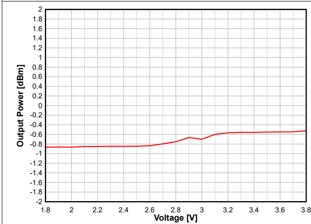
Figure 8-21. Output Power vs. Supply Voltage (VDD5) (BLE 1 Mbps, 2.44 GHz, 0 dBm)
