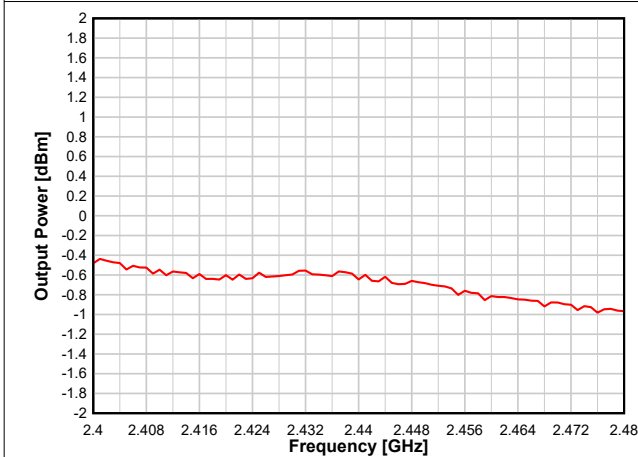
Figure 8-23. Output Power vs. Frequency (BLE 1 Mbps, 0 dBm)
