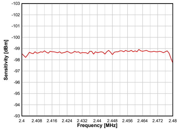
Figure 8-13. Sensitivity vs. Frequency (250 kbps)
