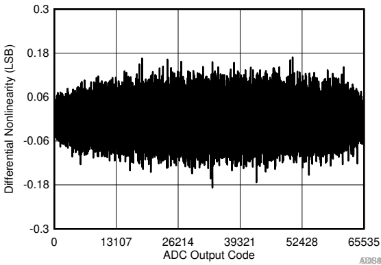
Figure 5-5. Typical DNL
