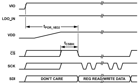
Figure 110. VIO POR Timing Diagram (Internal LDO Supplying VDD)
