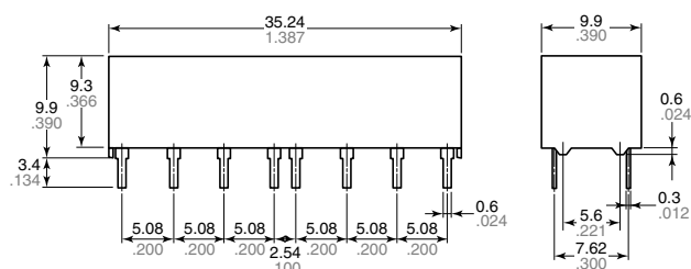
External dimensions
