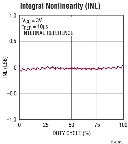
LTC2645-8 (Internal Reference, V FS = 2.5V)
