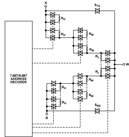
Figure 45. AD5121/AD5141 Simplified RDAC Circuit
