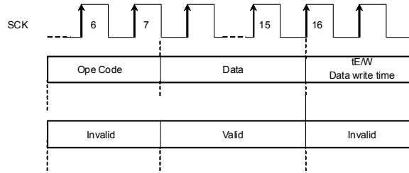
Figure 42. WPB valid timing (At inputting WRSR command)
