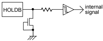
Figure 55. HOLDB input equivalent circuit
