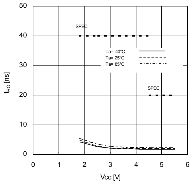
Figure 33. OUTPUT Rise Time vs Supply Voltage
