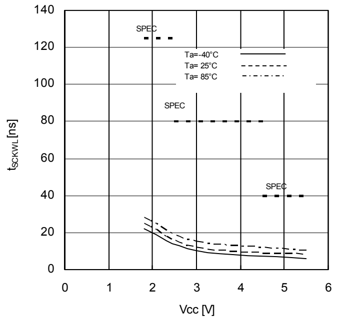
Figure 21. SCK Low Time vs Supply Voltage
