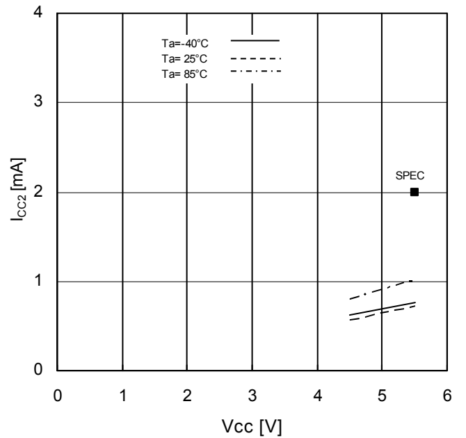
Figure 14. Supply Current (Write) vs Supply Voltage (fSCK=10MHz)
