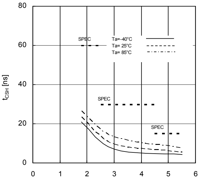
Figure 24. CSB Hold Time vs Supply Voltage
