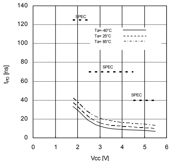
Figure 27. Data Output Delay Time vs Supply Voltage
