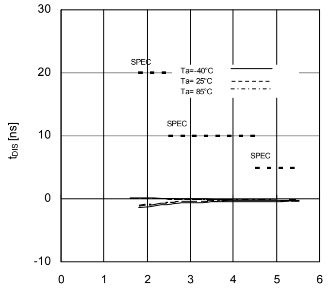
Figure 25. SI Setup Time vs Supply Voltage
