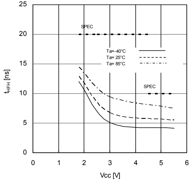
Figure 29. HOLDB Setting Hold Time vs Supply Voltage
