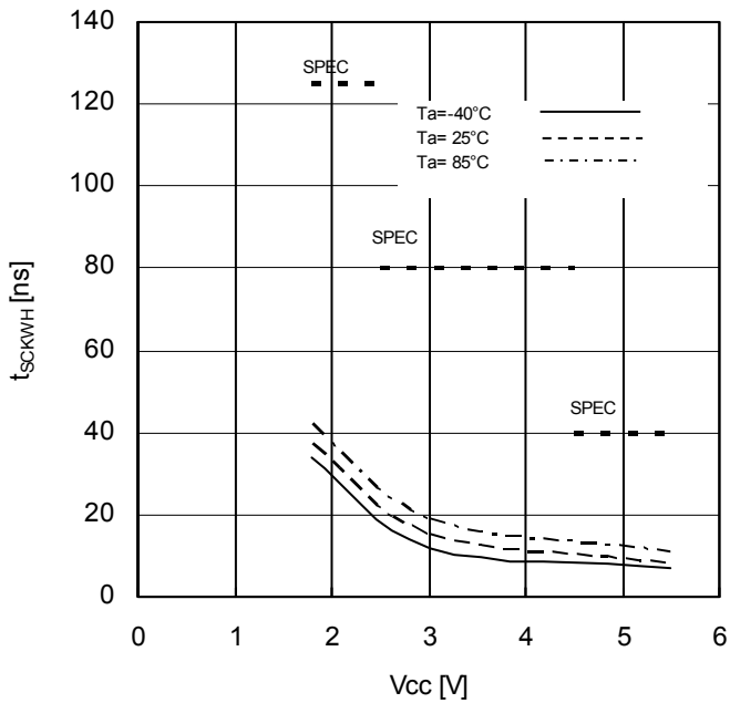
Figure 20. SCK High Time vs Supply Voltage
