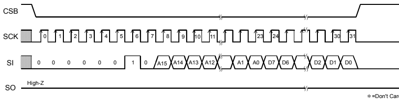
Figure 39. Write command
