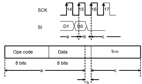
Figure 46. WRSR cancel valid timing
