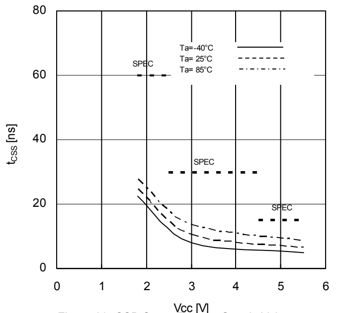
Figure 23. CSB Setup Time vs Supply Voltage
