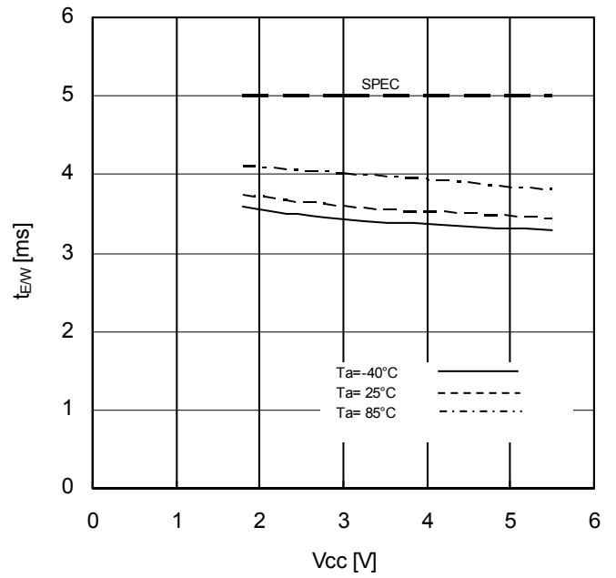
Figure 35. Write Cycle Time vs Supply Voltage
