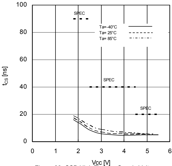
Figure 22. CSB High Time vs Supply Voltage
