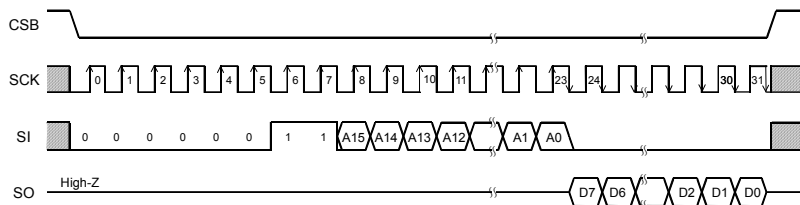
Figure 38. Read command
