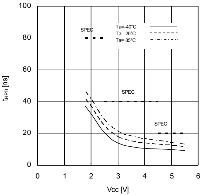
Figure 32. Time from HOLDB to Output change vs Supply Voltage
