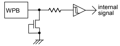
Figure 56. WPB input equivalent circuit
