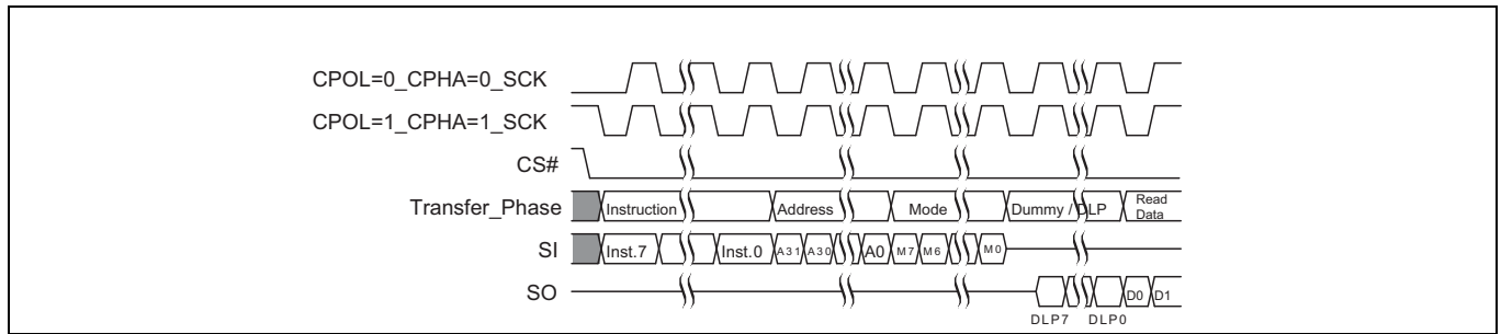
Figure 6 SPI DDR modes supported
