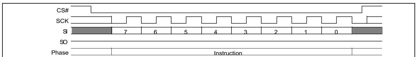
Figure 52 BRAC (B9h) command sequence
