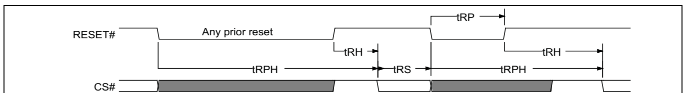
Figure 29 Hardware reset
