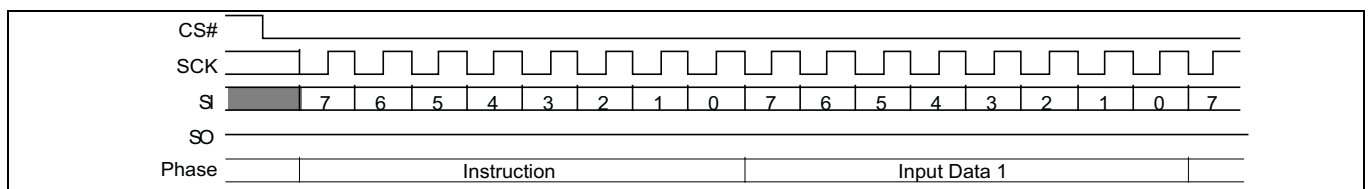
Figure 62 AutoBoot register write (ABWR) Command
