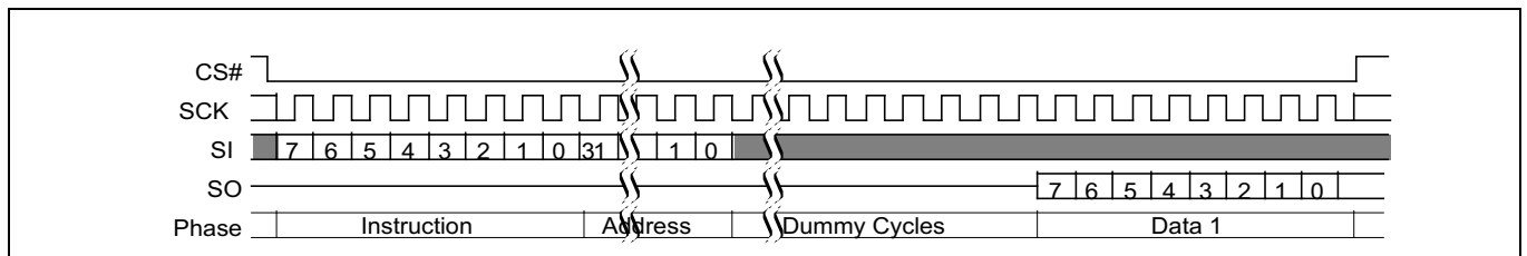
Figure 11 Single bit wide I/O command with latency
