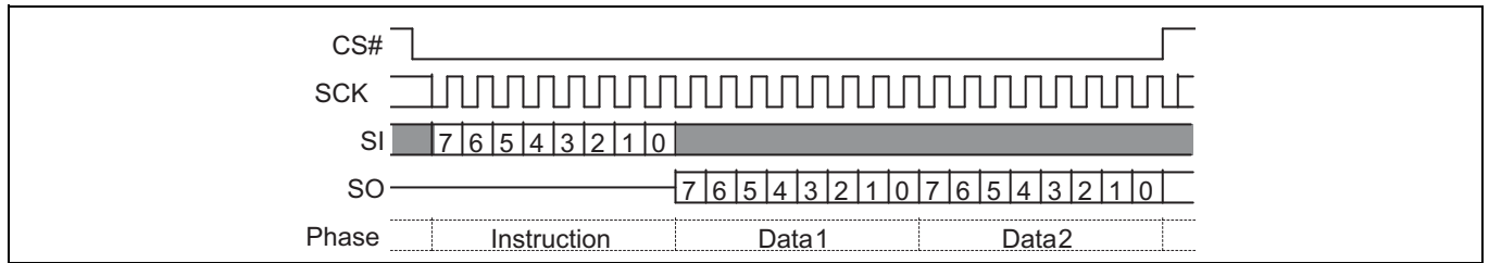
Figure 9 Single bit wide output command
