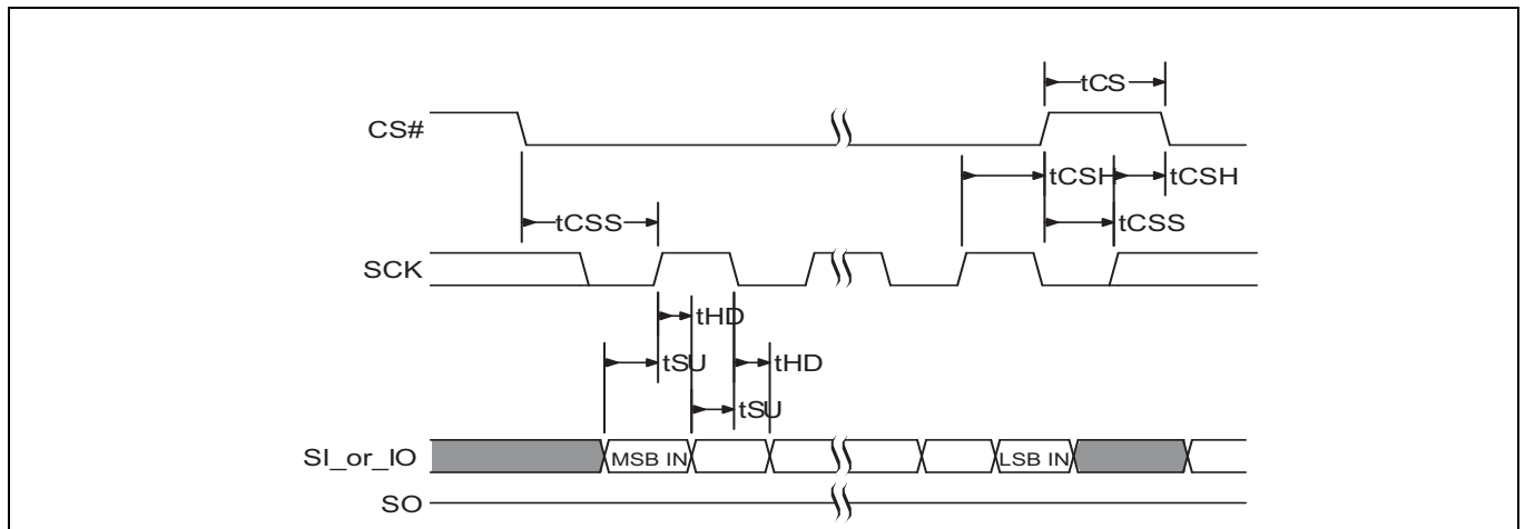
Figure 36 SPI DDR input timing
