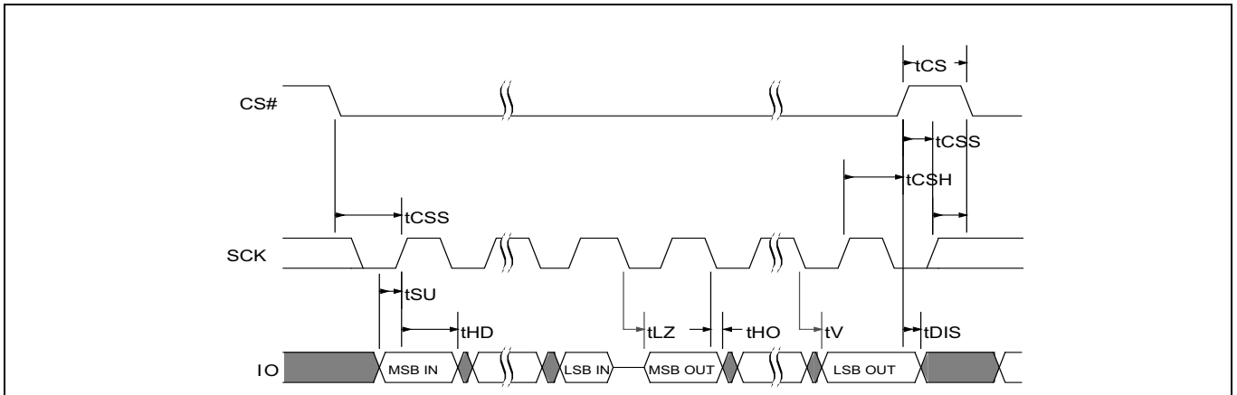
Figure 33 SPI SDR MIO timing
