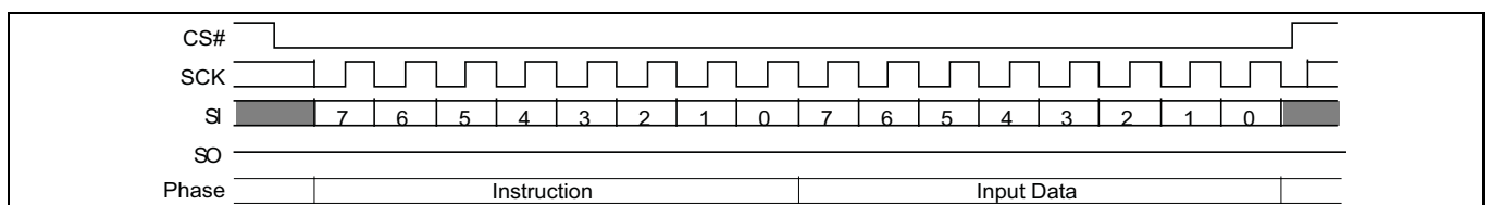
Figure 63 Program NVDLR (PNVDLR 43h) command sequence
