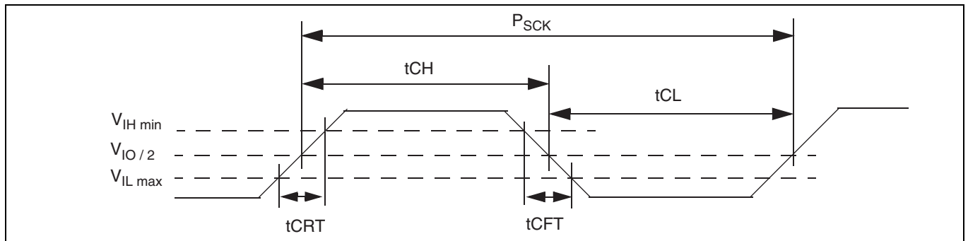
Figure 30 Clock timing
