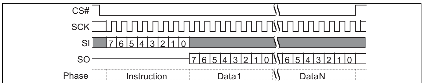
Figure 61 AutoBoot register read (ABRD 14h) Command
