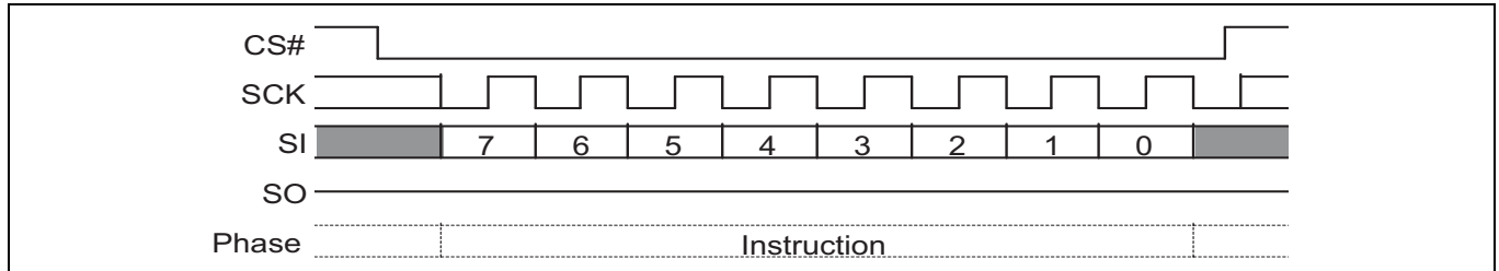
Figure 55 Write enable (WREN 06h) command sequence
