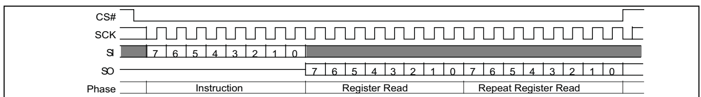
Figure 50 Read bank register (BRRD 16h) command
