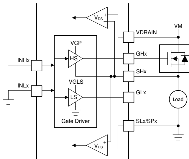
Figure 13-6. Single High-Side Driver
