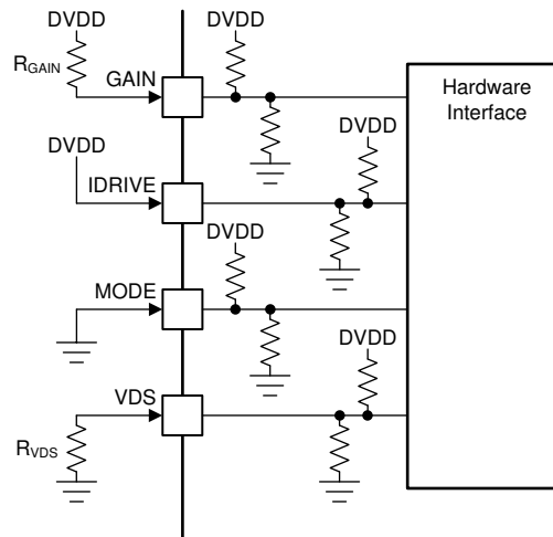
Figure 13-9. Hardware Interface
