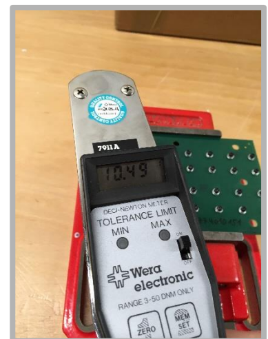
Digital torque wrench for Breaking Torque
