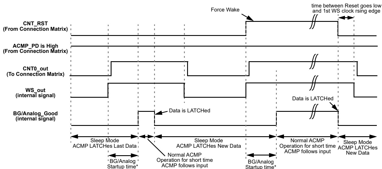
Figure 95: Wake/Sleep Timing Diagram, Short Wake Mode, Counter Reset is Used
