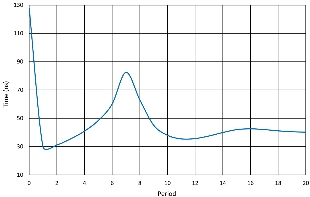
Figure 138: Oscillator1 Settling Time, V_{DD} = 3.3 V, T = 25 °C, OSC1 = 25 MHz (Start with Delay)
