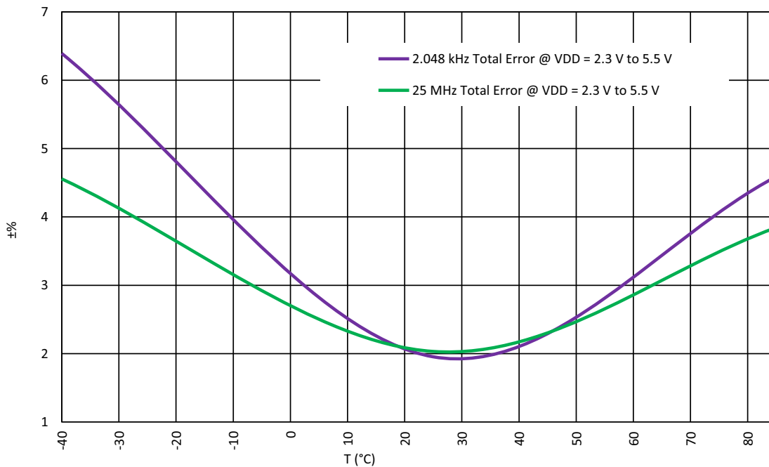
Figure 135: Oscillators Total Error vs. Temperature
