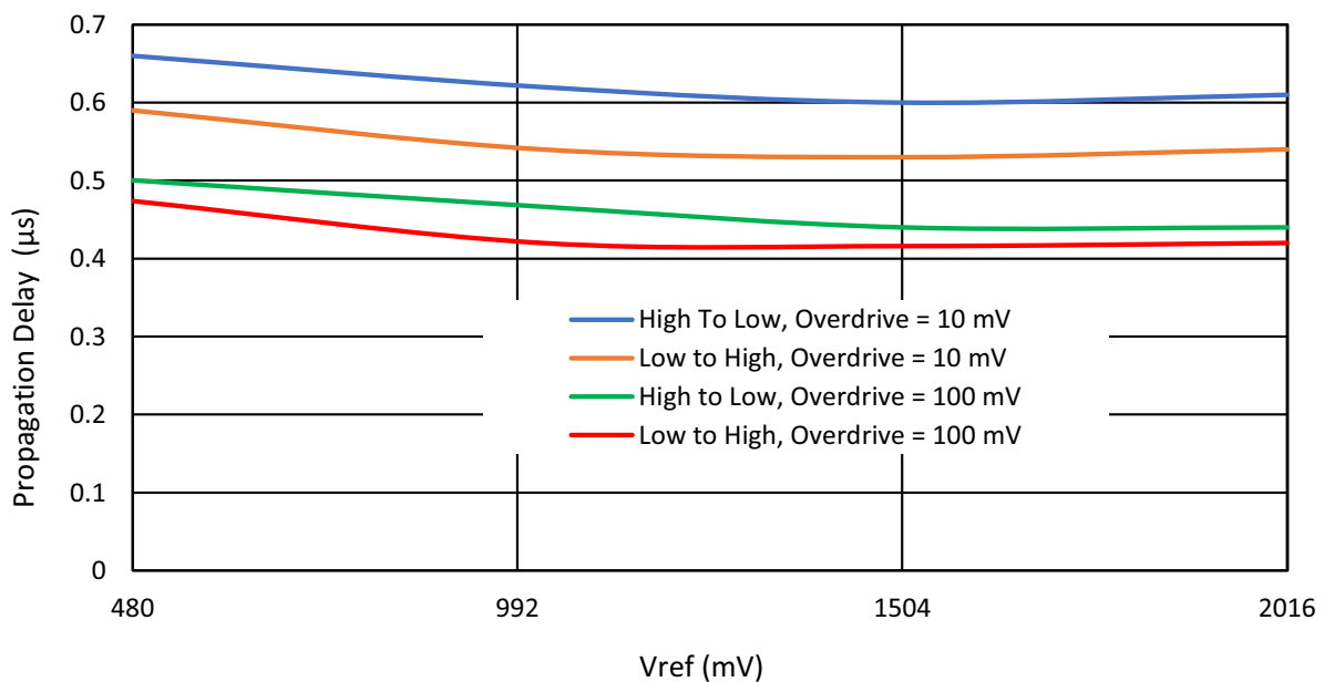
Figure 44: Typical Propagation Delay vs. Vref for CCMPx at T = 25\text{ }^{\circ}\text{C} , at V_{DD} = 2.3\text{ V} to 5.5\text{ V} , Gain = 4
