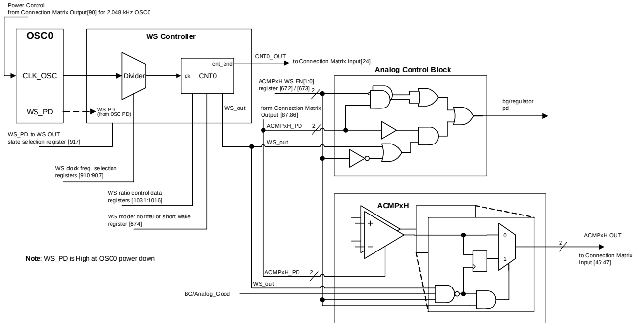
Figure 93: Wake/Sleep Controller
