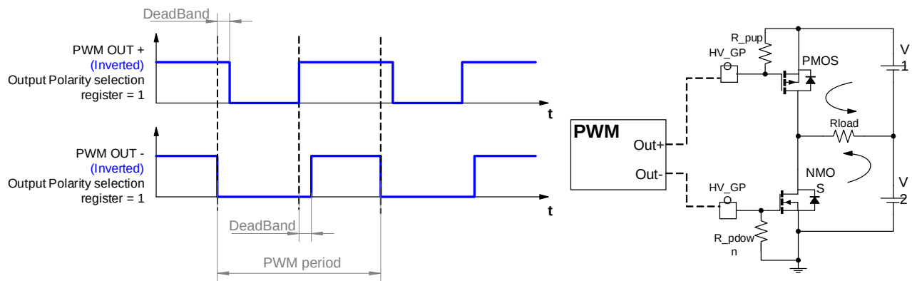
Figure 99: PWM Output Waveforms and Test Circuit Example for Driving NMOS and PMOS FETs
