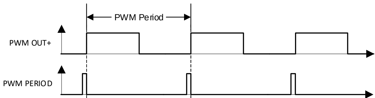
Figure 107: PWM Period Waveform
