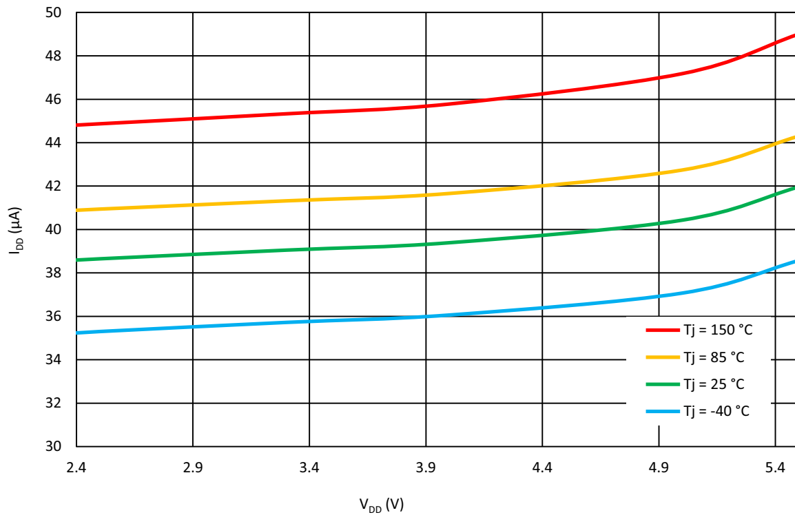
Figure 116: ACMPxH Current Consumption vs. V_{DD} at V_{ref} = 1024 \text{ mV}
