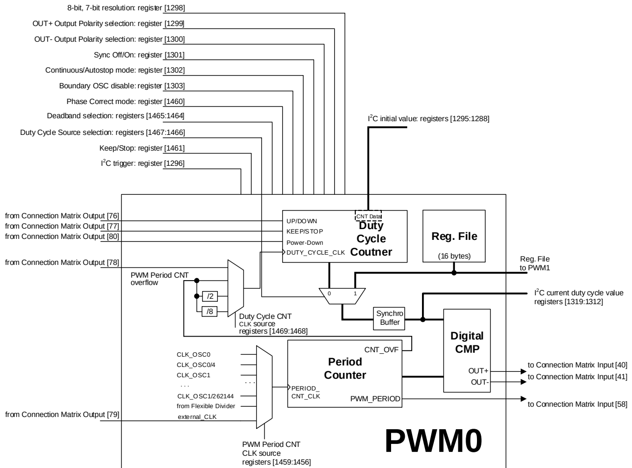
Figure 108: PWM0 Functional Diagram
