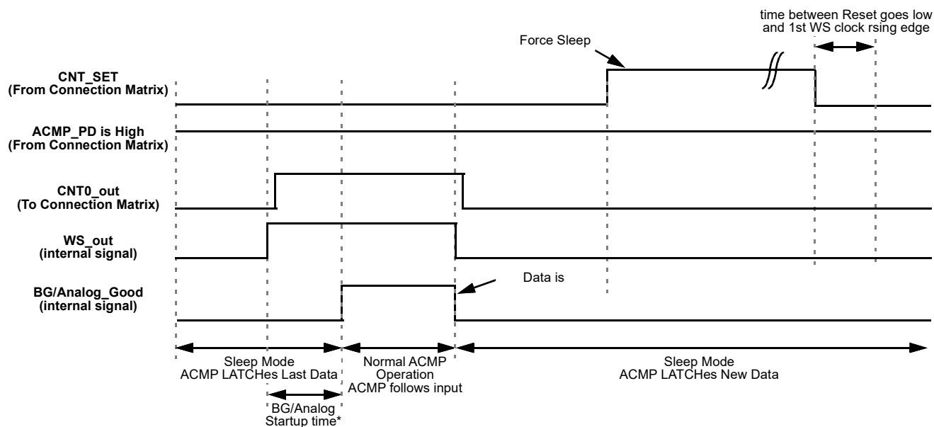
Figure 96: Wake/Sleep Timing Diagram, Normal Wake Mode, Counter Set is Used
