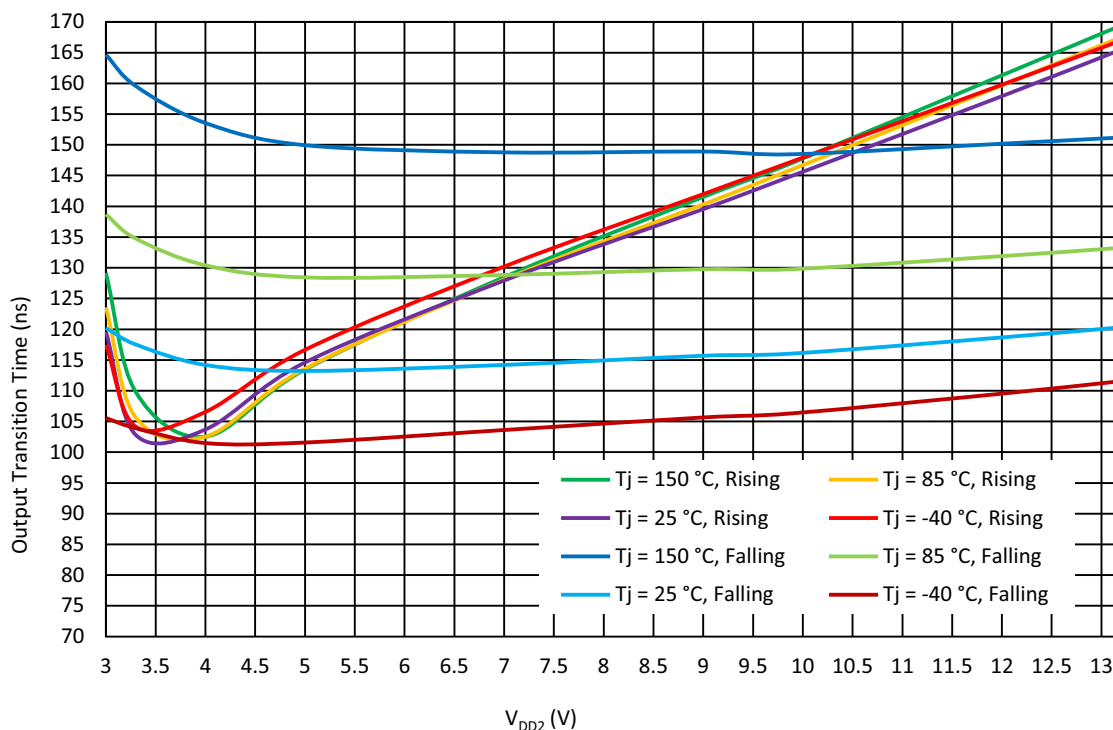
Figure 33: Half Bridge Output Transition Time vs. V_{DD2} at V_{DD} = 2.3\text{ V} to 5.5\text{ V} , f = 50\text{ kHz} for Regular Mode
