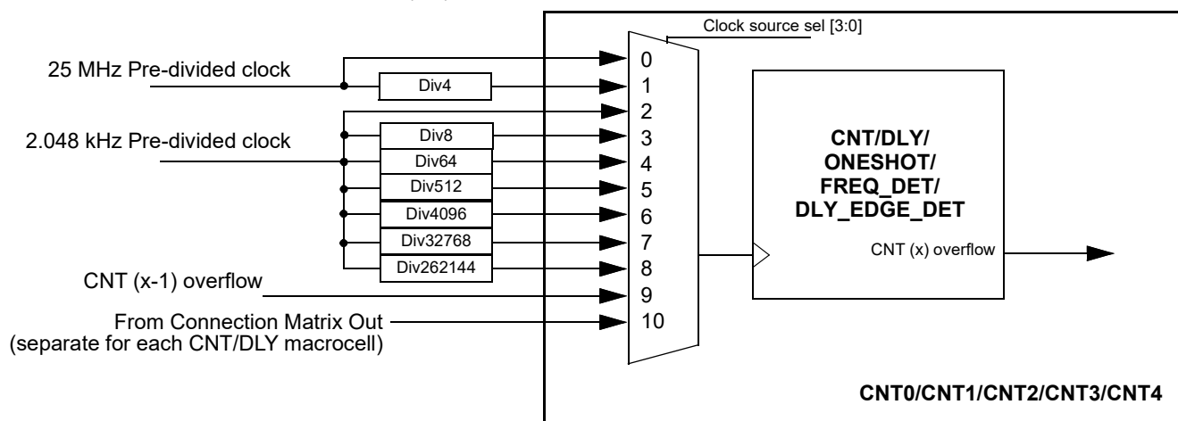
Figure 128: Clock Scheme
