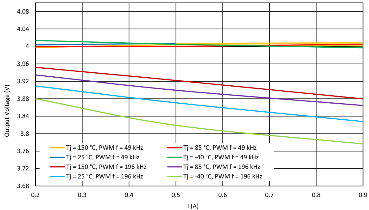
Figure 40: Typical Load Regulation at V_{OUT} = 4.096 V, V_{DD} = 2.3 V to 5.5 V, V_{DD2} = 9 V
