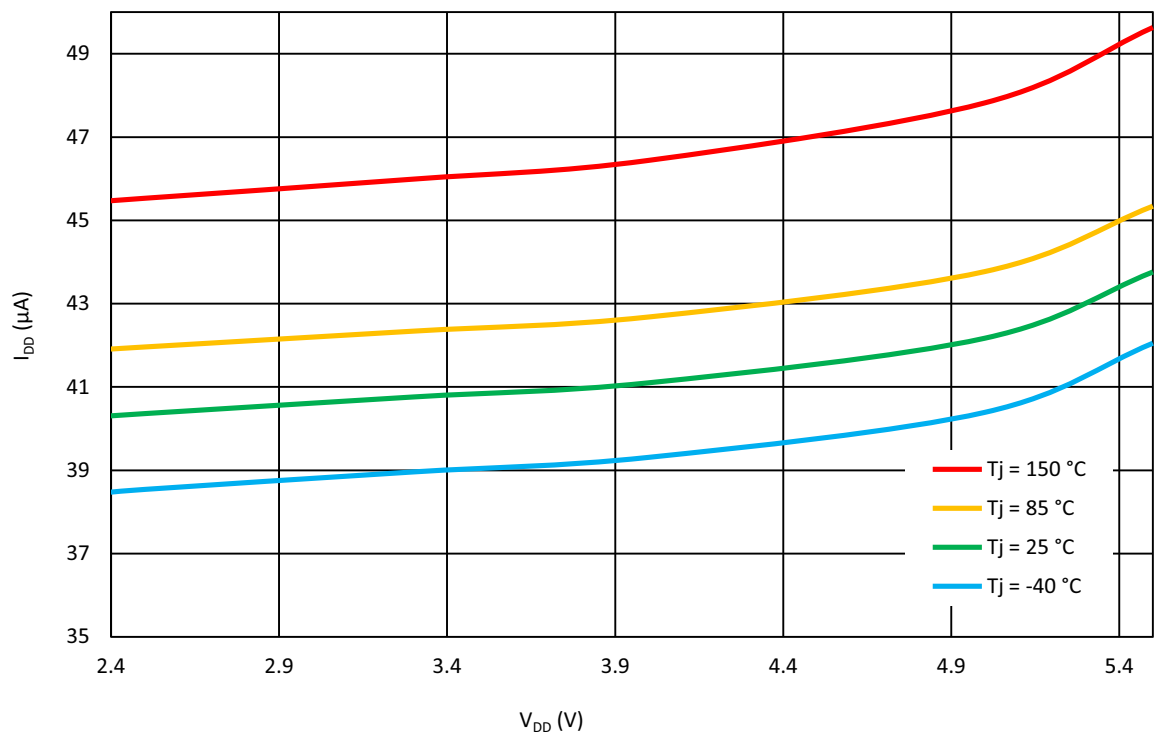
Figure 117: ACMPxH Current Consumption vs. V_{DD} at V_{ref} = 2016 \text{ mV}
