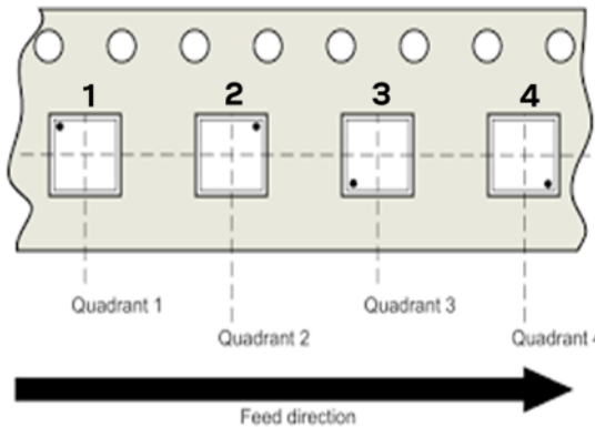
Figure 10: Carrier tape quadrants
