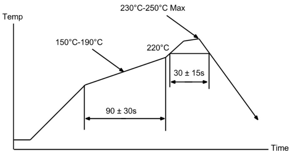
Figure 11: Reflow profile for lead free solder
