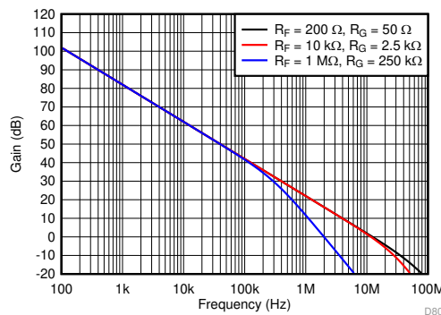
Figure 67. Loop-Gain vs. Frequency for Circuit of Figure 66
