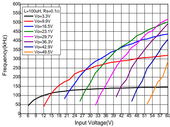
Operating Frequency vs. Input Voltage ( R_s=0.1\Omega , L=100\mu\text{H} )
