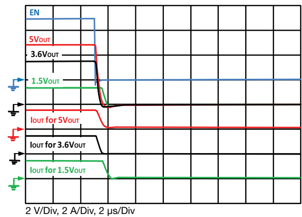
Fig. 20 - Typical Fall Time C_{OUT} = 0.1 \mu F , C_{IN} = 4.7 \mu F , I_{OUT} = 1.5 A
