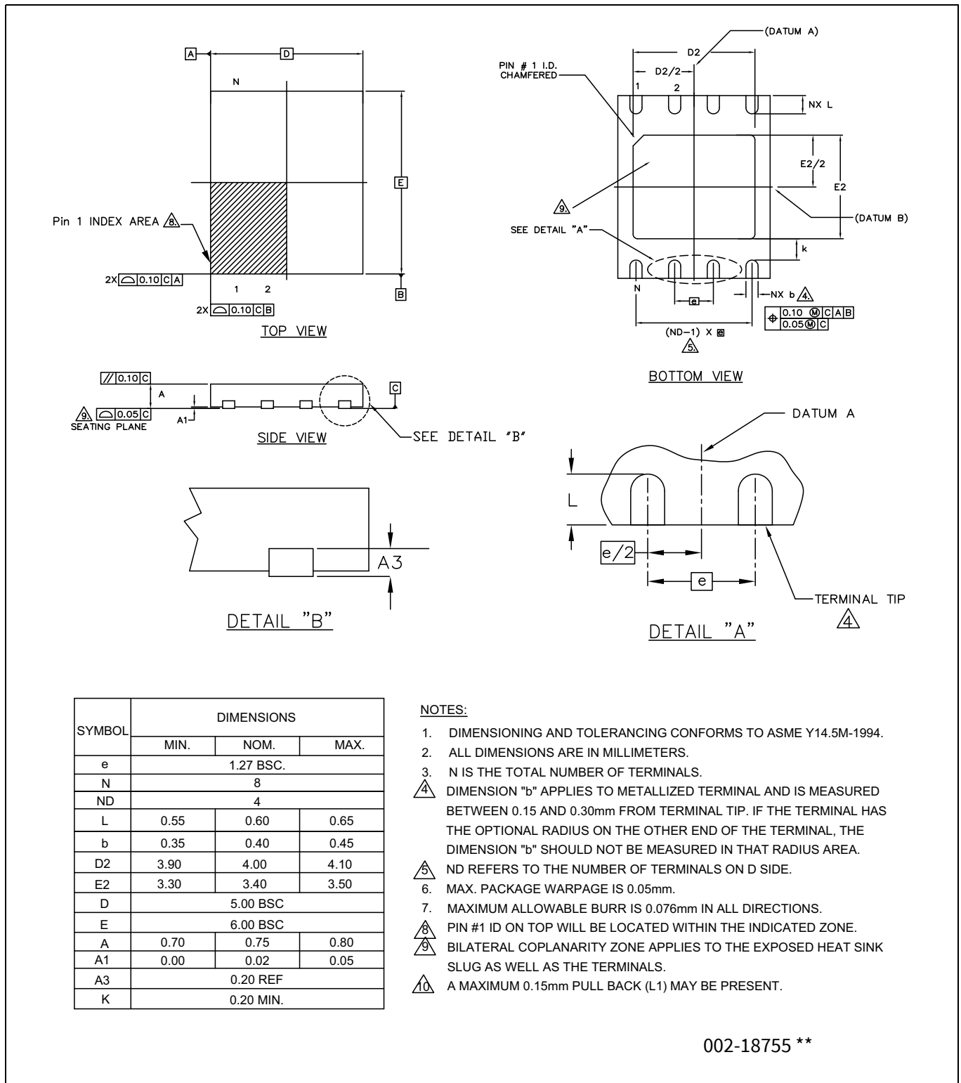
Figure 39 8-lead DFN (5.0 x 6.0 x 0.8 mm) package outline, 002-18755
