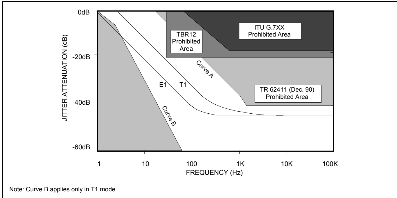
Figure 10-74. Jitter Attenuation
