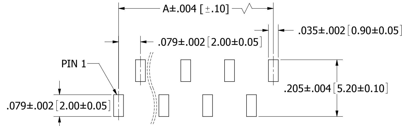
RECOMMENDED PCB LAYOUT - FOR PN: xPxNxx1BFLD-RC
