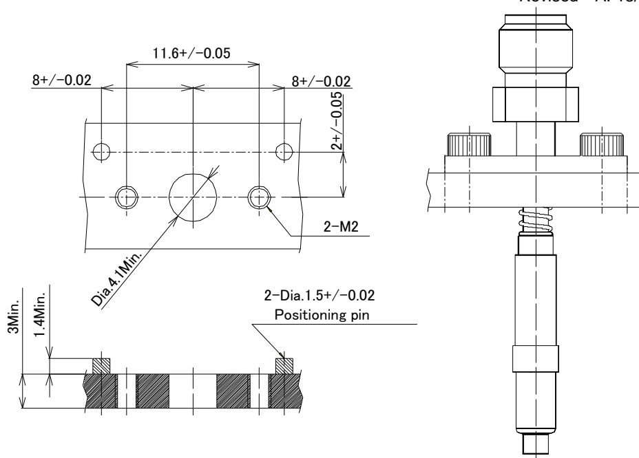
Figure.5 Machine's hole diameter for attachment probe
