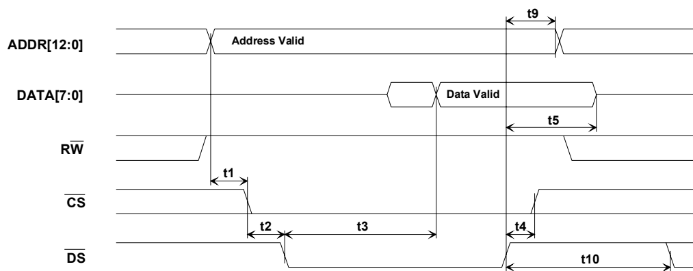
Figure 11-11 Motorola Bus Read Timing (HWMODE = 0, MODEC = 01)
