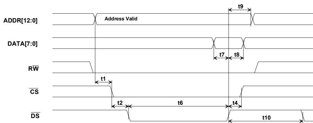
Figure 11-12 Motorola Bus Write Timing (HWMODE = 0, MODEC = 01)
