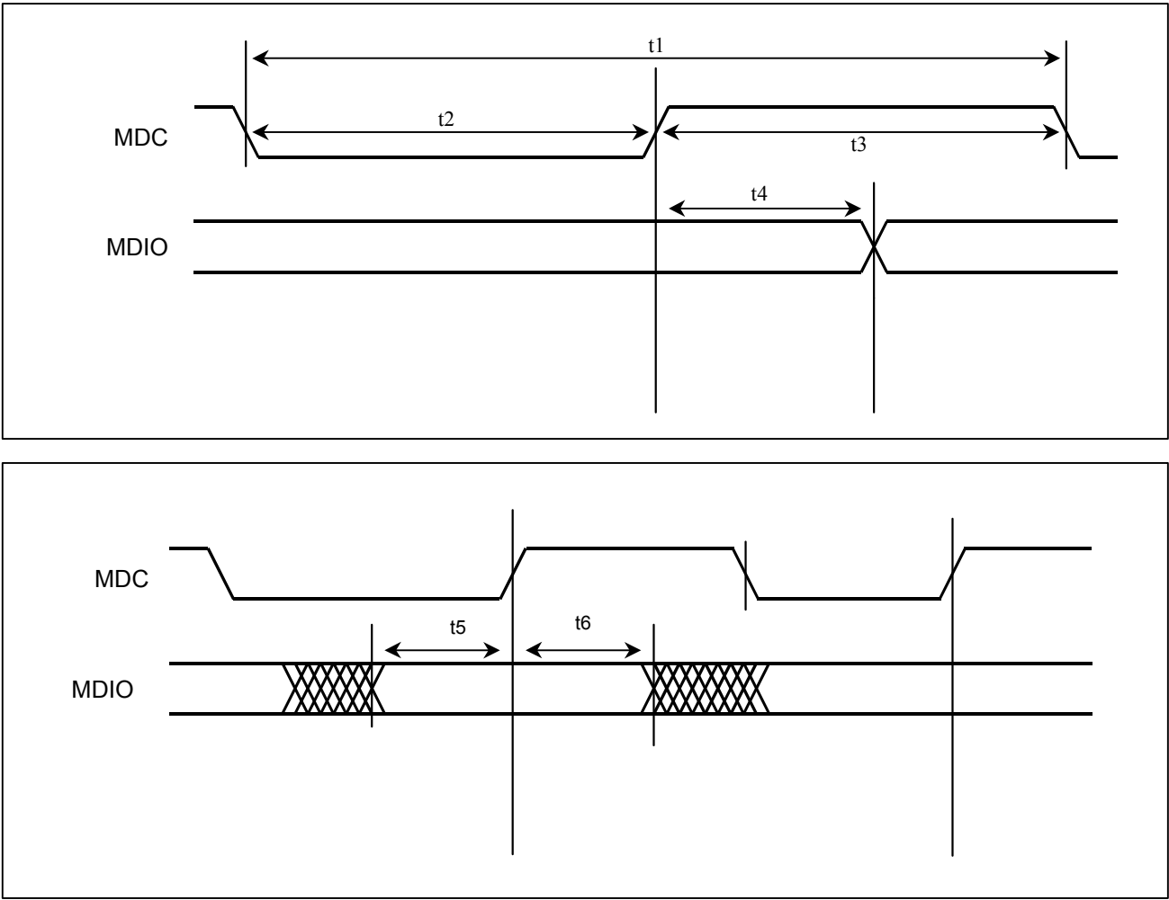
Figure 11-5 MDIO Timing
