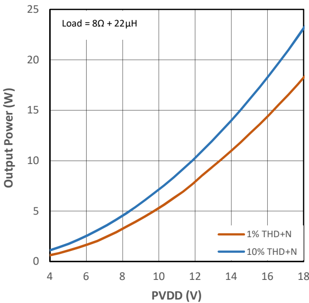
Figure 11-23 Output Power vs PVDD Voltage for PMP2
