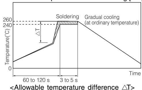
Recommended profile for Flow soldering [Ex.]
