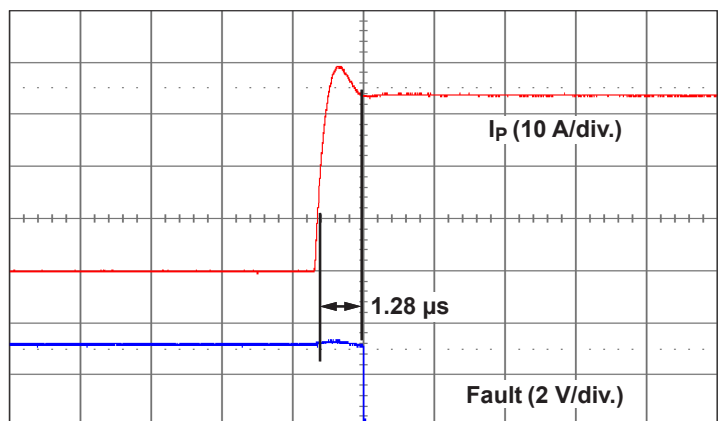
Fault Response
